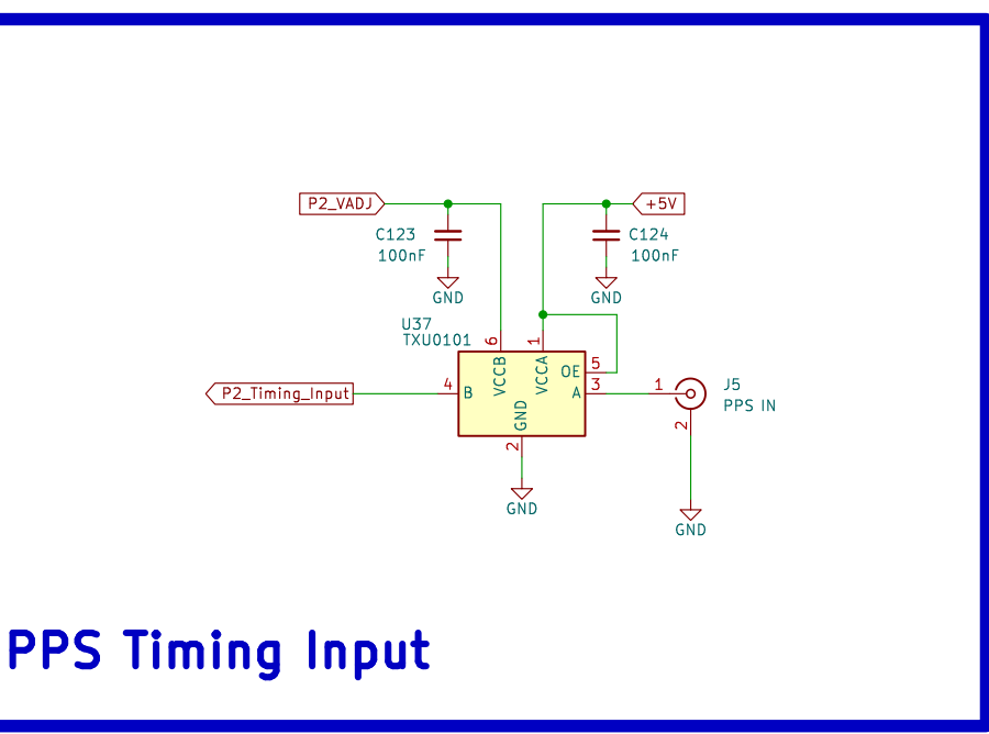
Level Shifters
