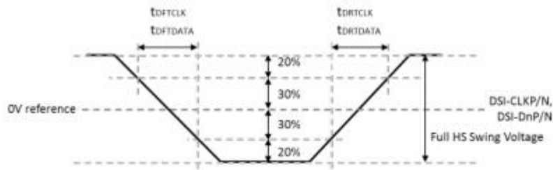
Figure 6-2 Rising and Falling Timings
