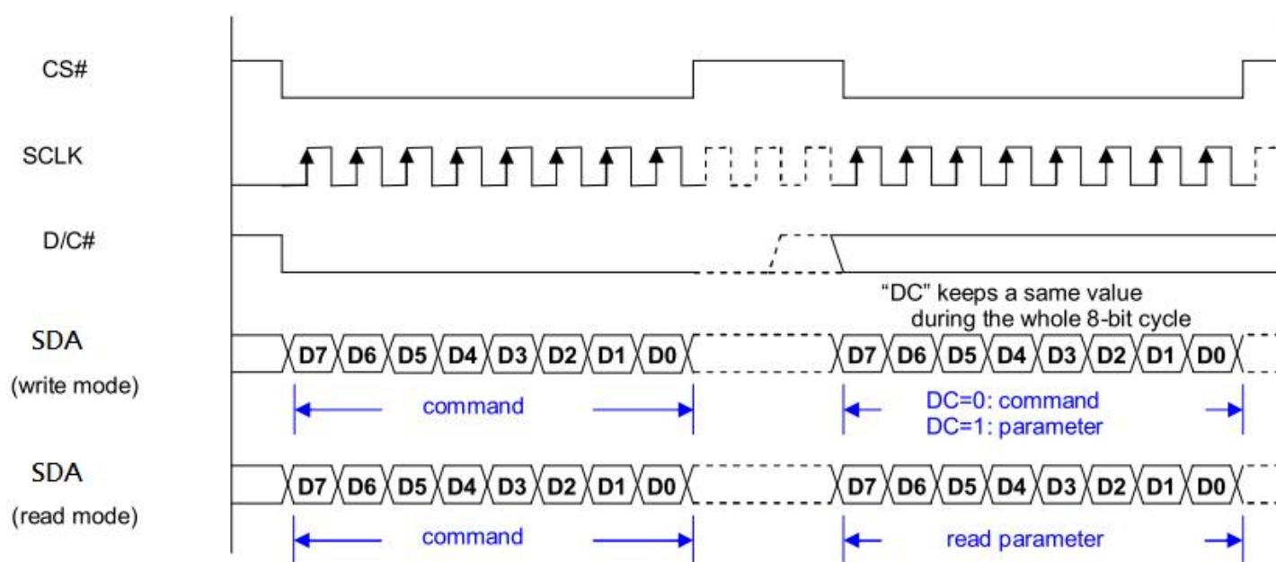
Figure 5-1 Write procedure in 4-wire SPI mode
