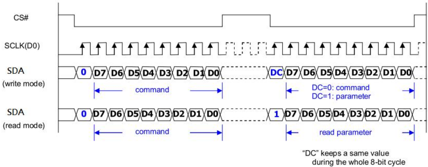
Figure 5-2 Write procedure in 3-wire SPI mode
