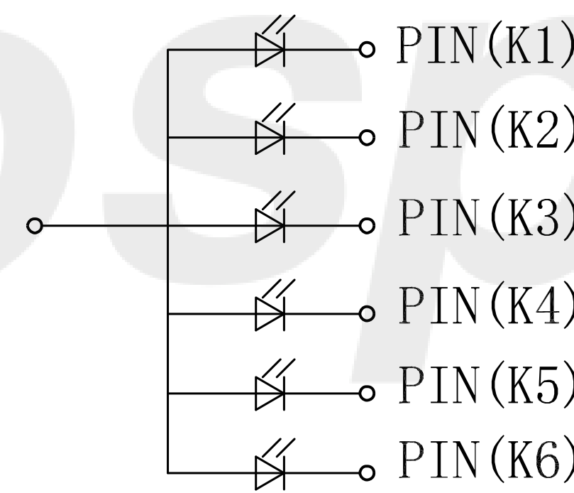
LED CIRCUIT DIAGRAM VF=3.0±0.2V IF=120mA
