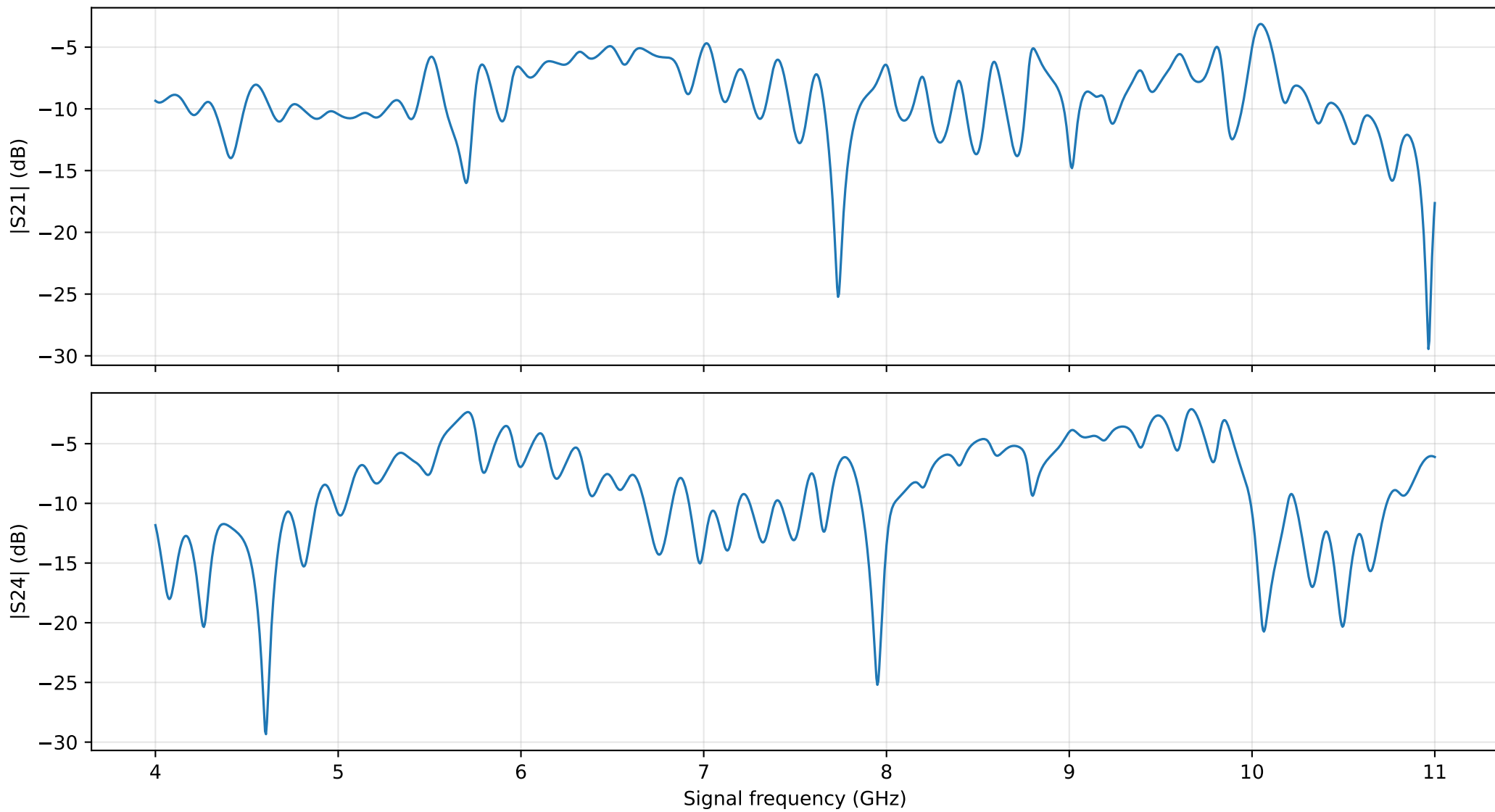
Pump-off response: ipm_7c_fixed
