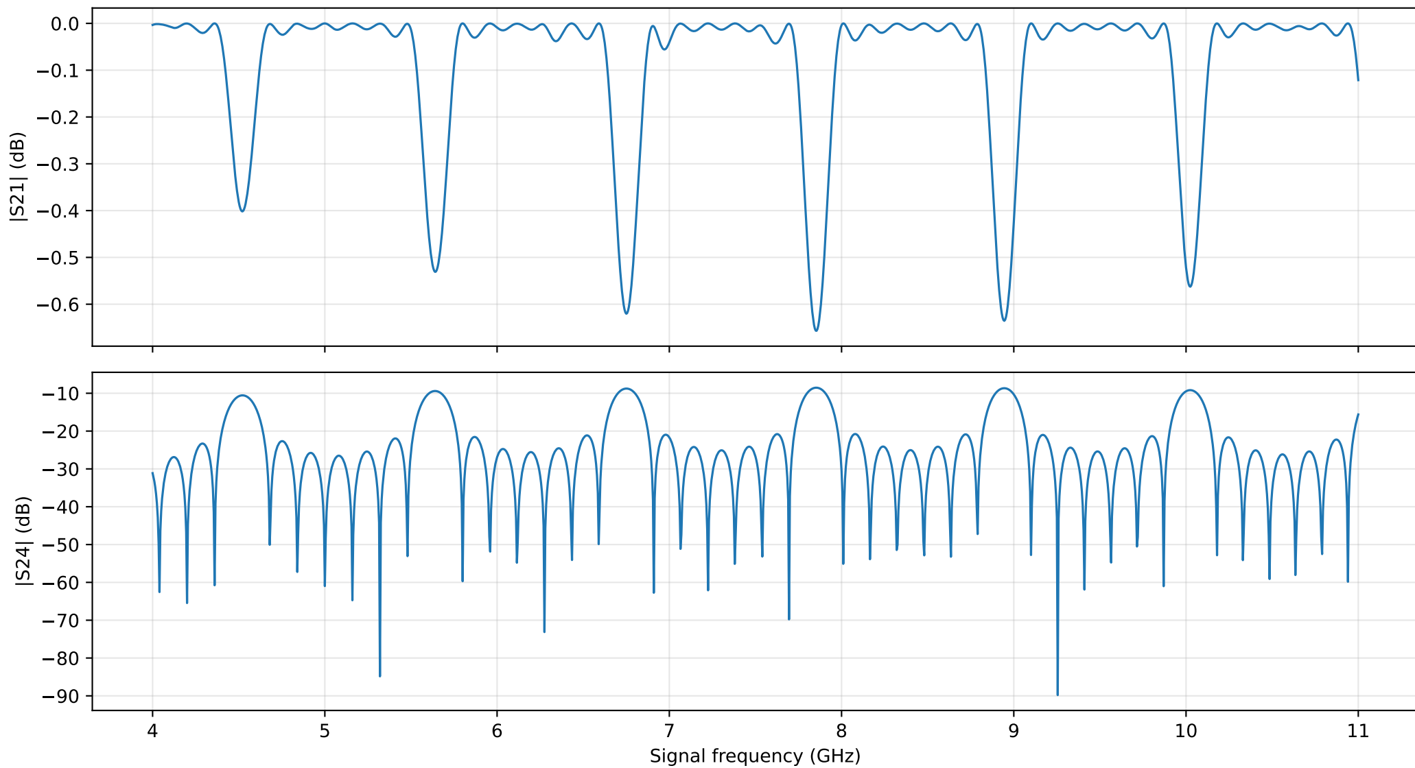
Pump-off response: ipm_7c_ideal_m25db_8ghz
