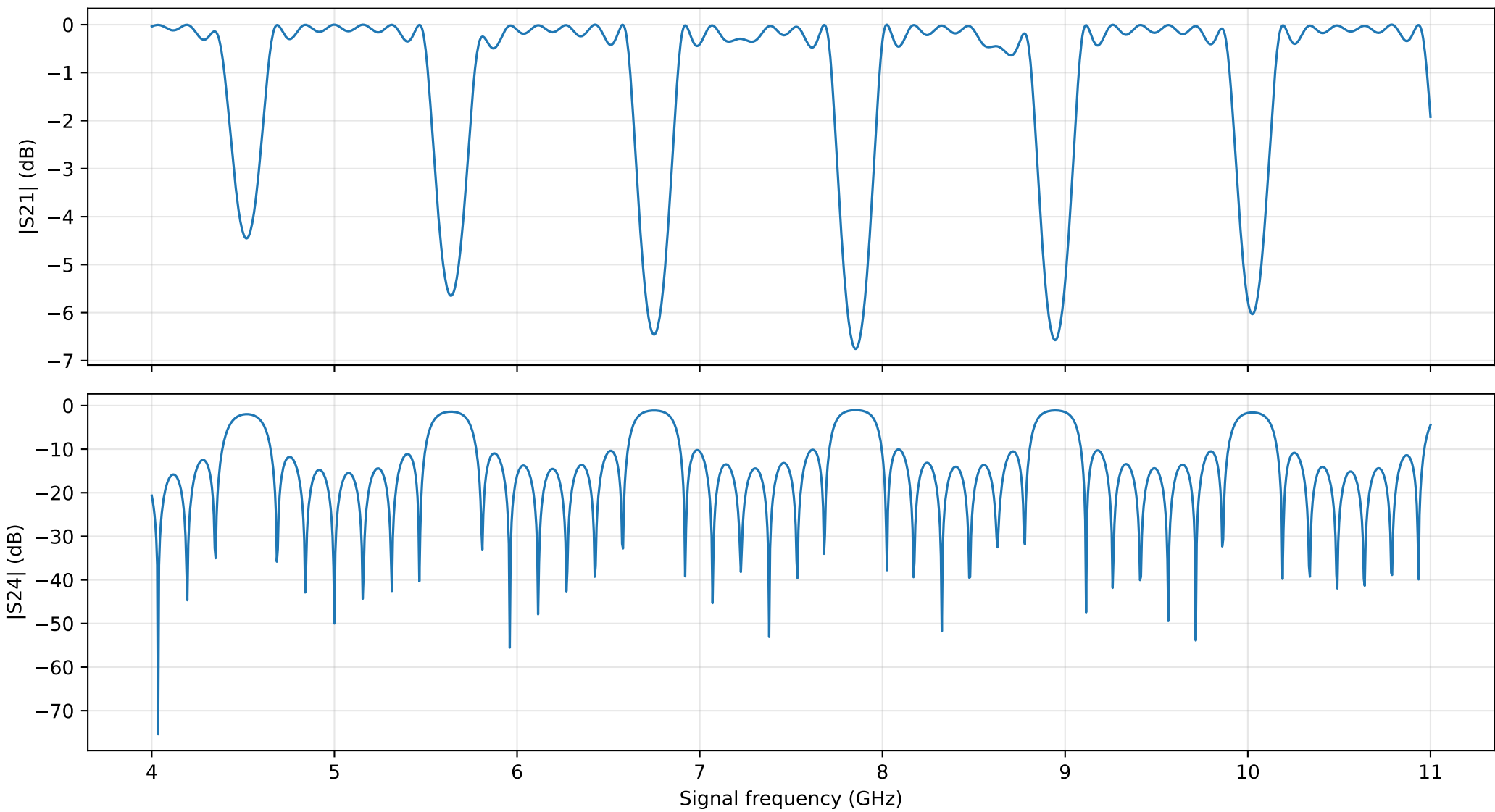
Pump-off response: ipm_7c_new
