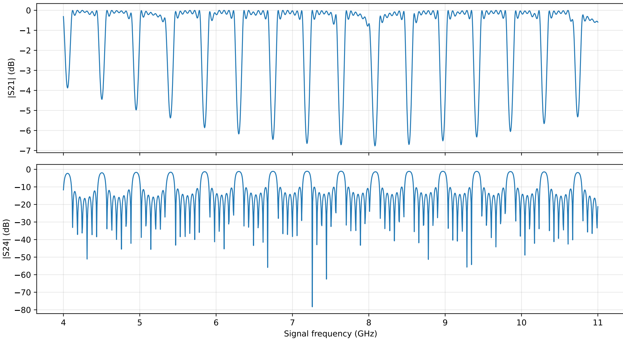
Pump-off response: ipm_7c_old
