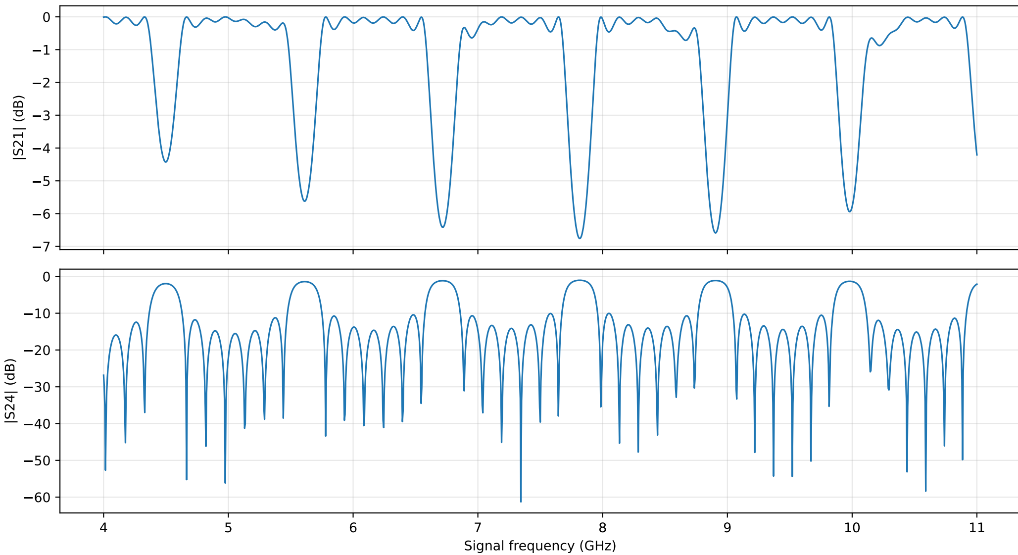
Pump-off response: ipm_7c_oldlen_newcl
