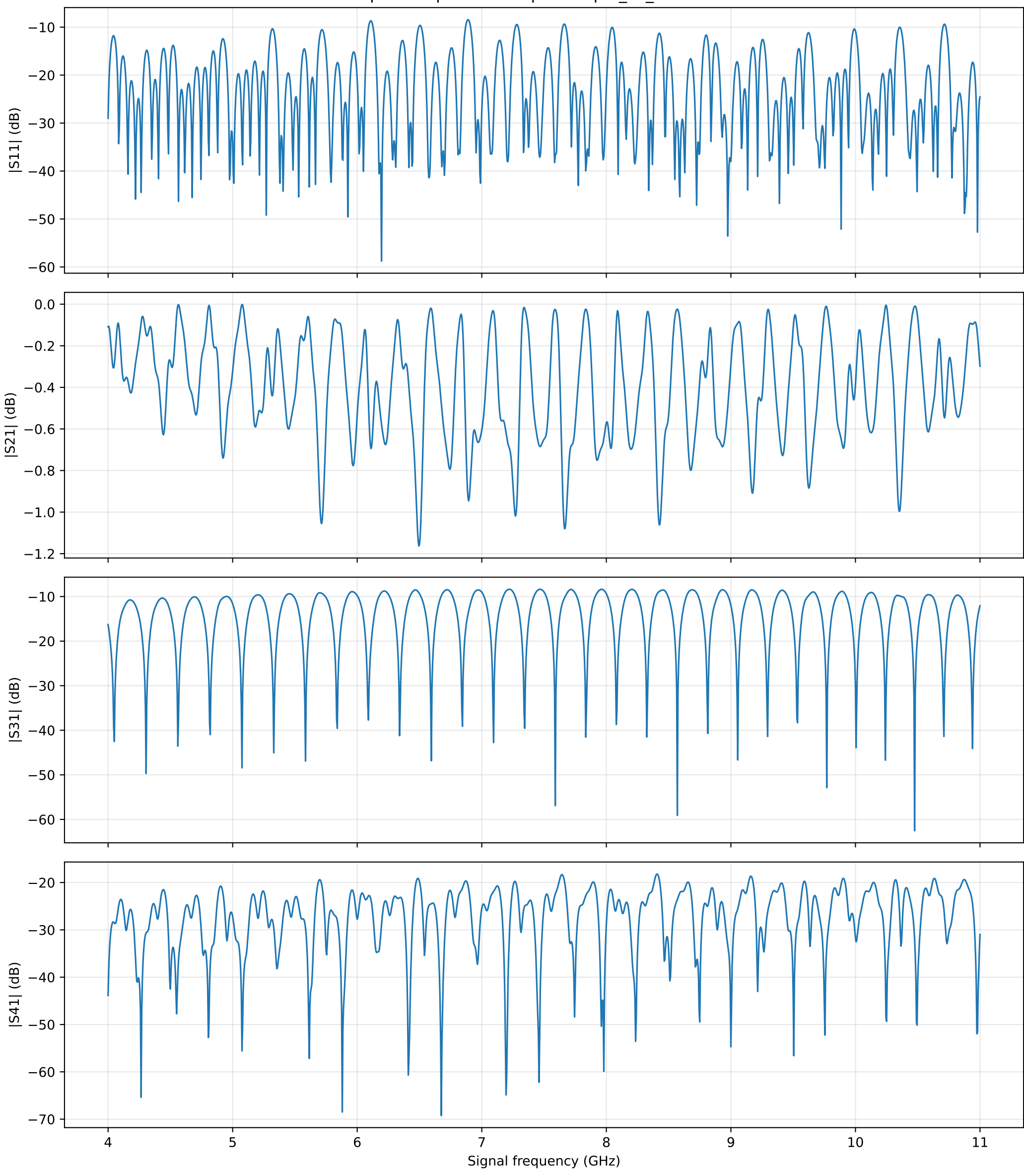
Pump-off response from port 1: ipm_2c_fixed
