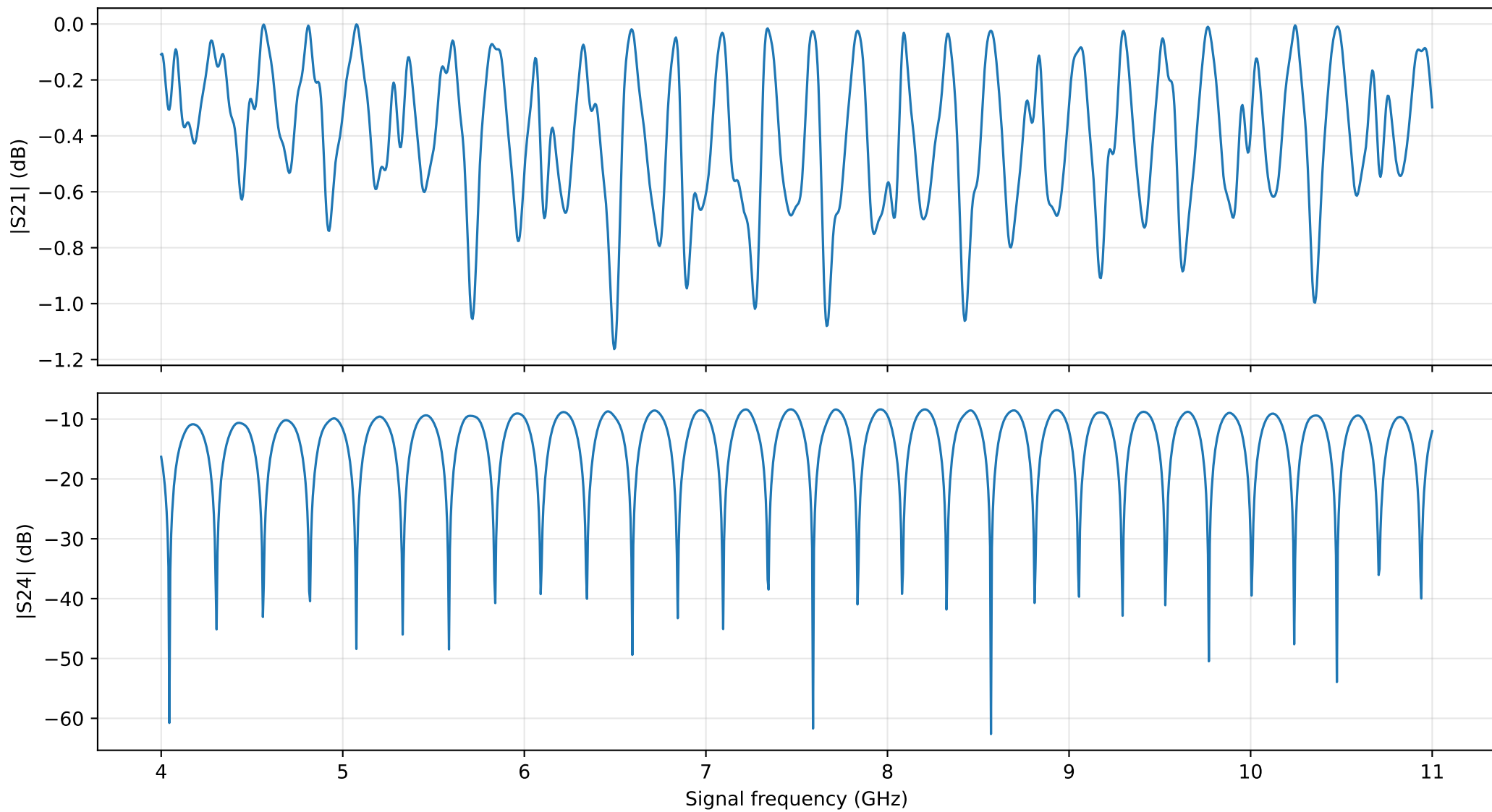
Pump-off response: ipm_2c_fixed
