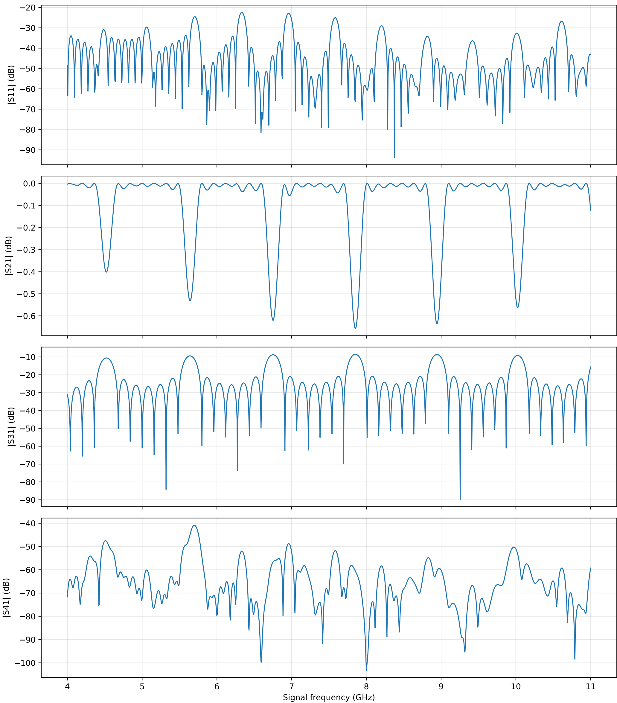
Pump-off response from port 1: ipm_7c_ideal_m25db_8ghz
