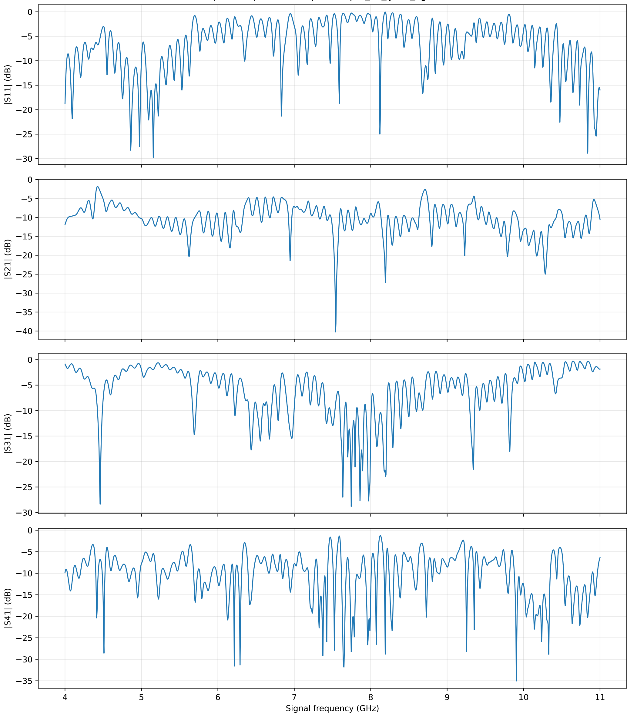
Pump-off response from port 1: ipm_7c_lj158_cg66
