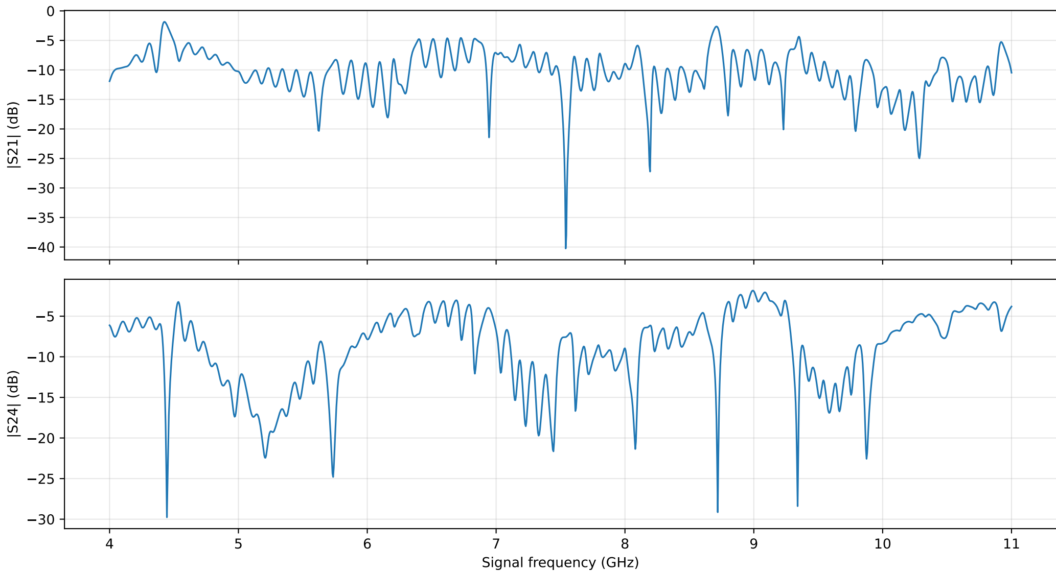
Pump-off response: ipm_7c_lj158_cg66
