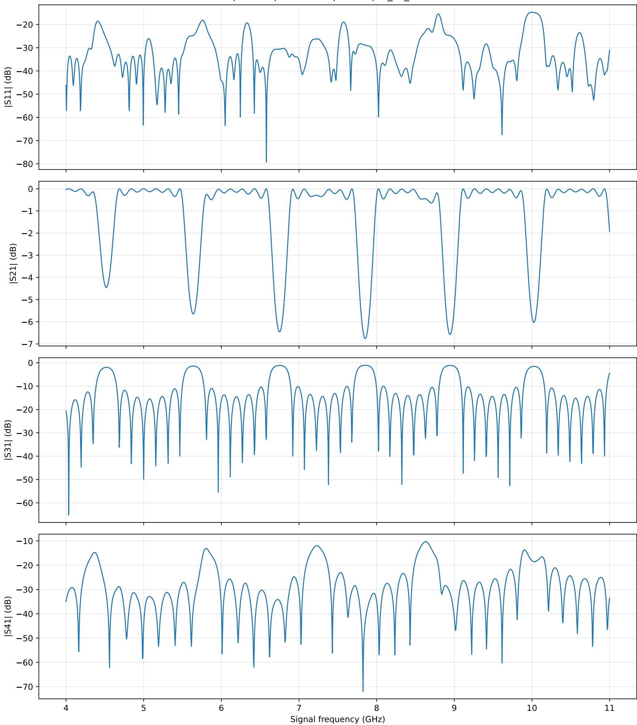
Pump-off response from port 1: ipm_7c_new
