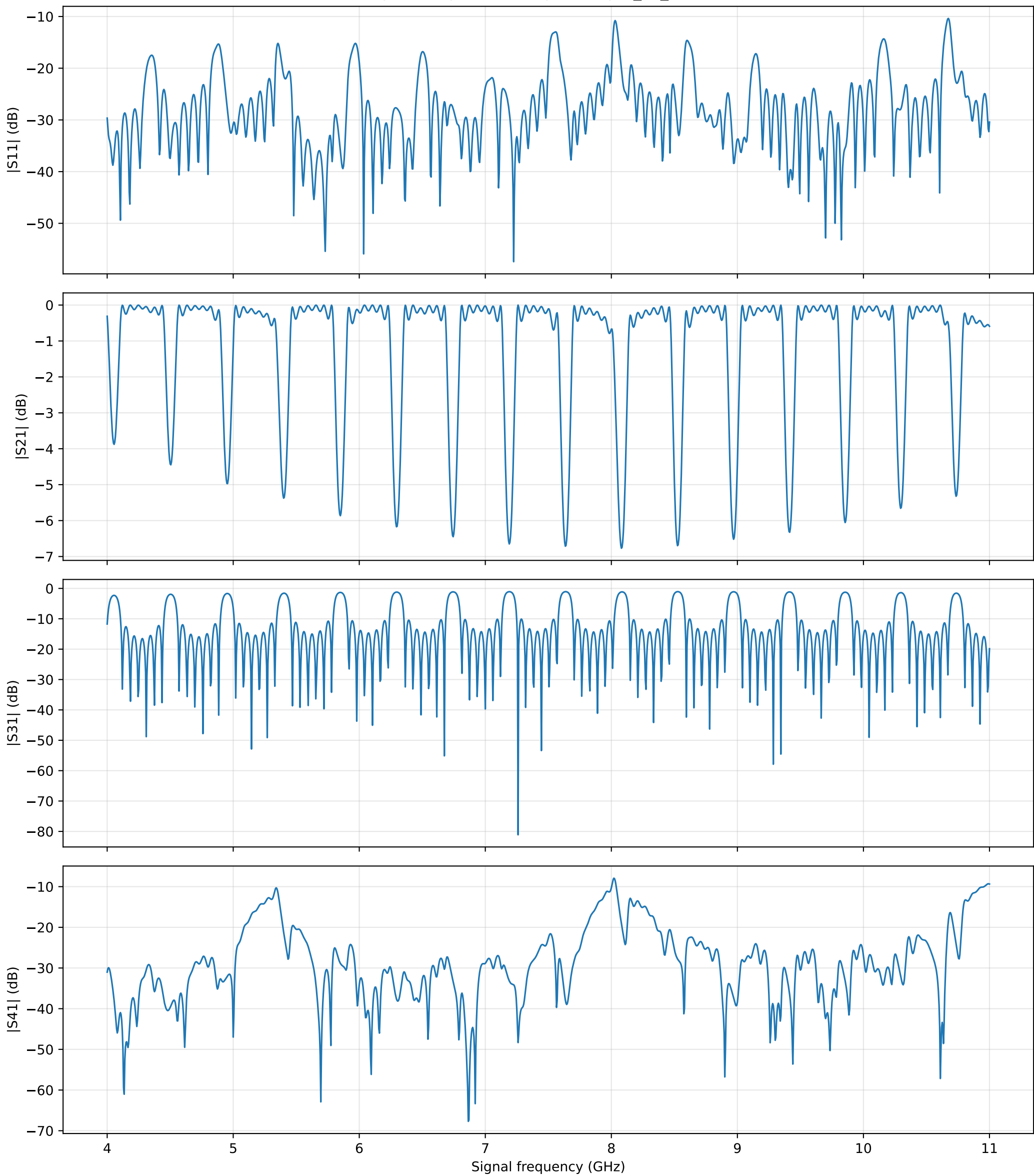
Pump-off response from port 1: ipm_7c_old
