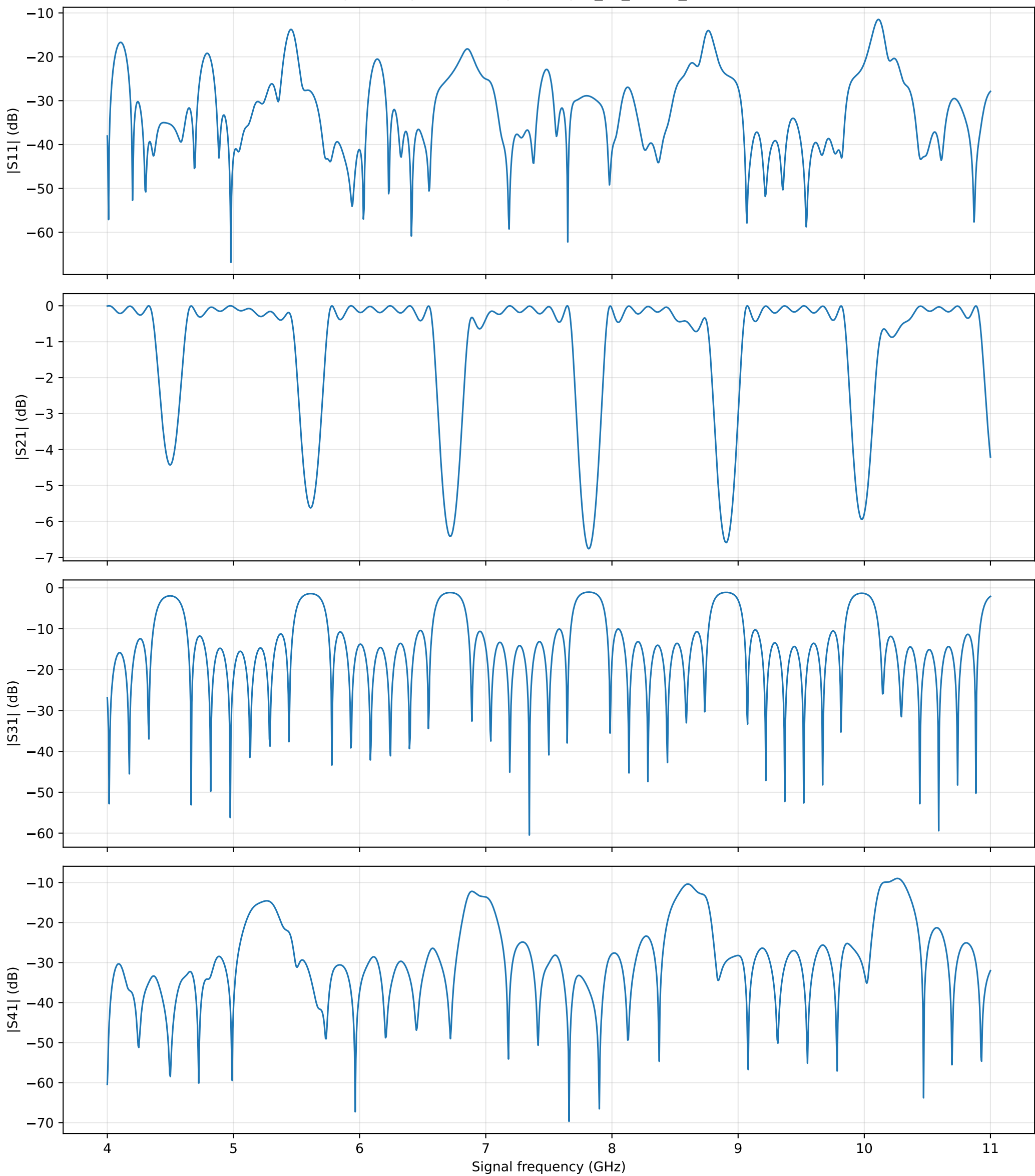
Pump-off response from port 1: ipm_7c_oldlen_newcl
