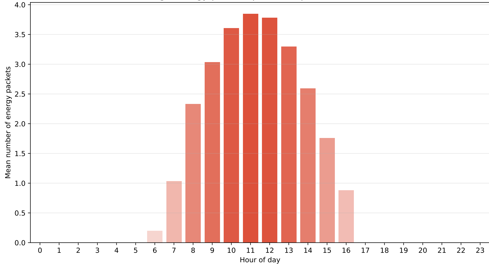
Santiago - Regime M2 (Partly cloudy) Average energy packets per hour (packet = 800 Wh)
