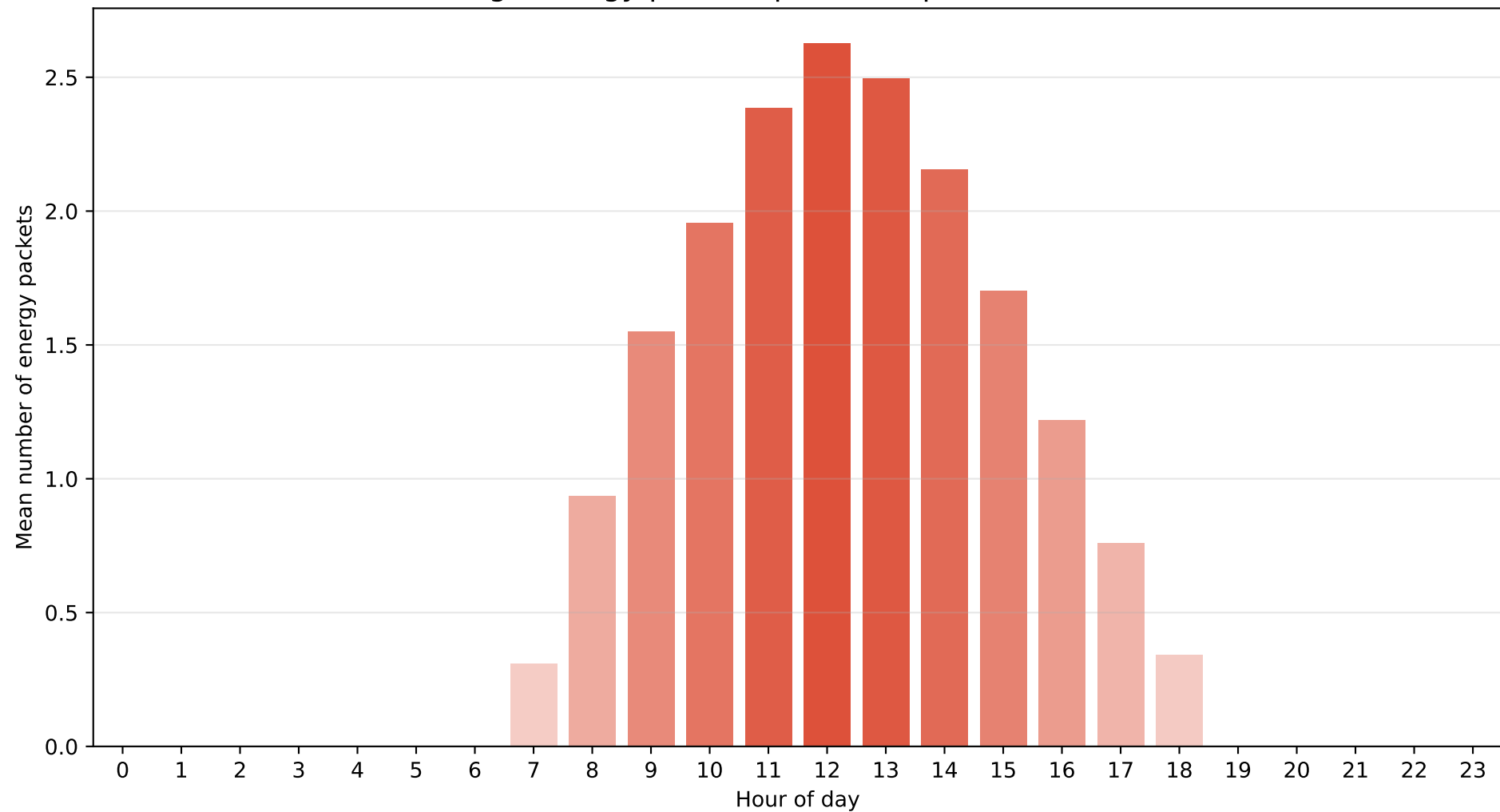
Paris – Regime M2 (Partly cloudy) Average energy packets per hour (packet = 800 Wh)
