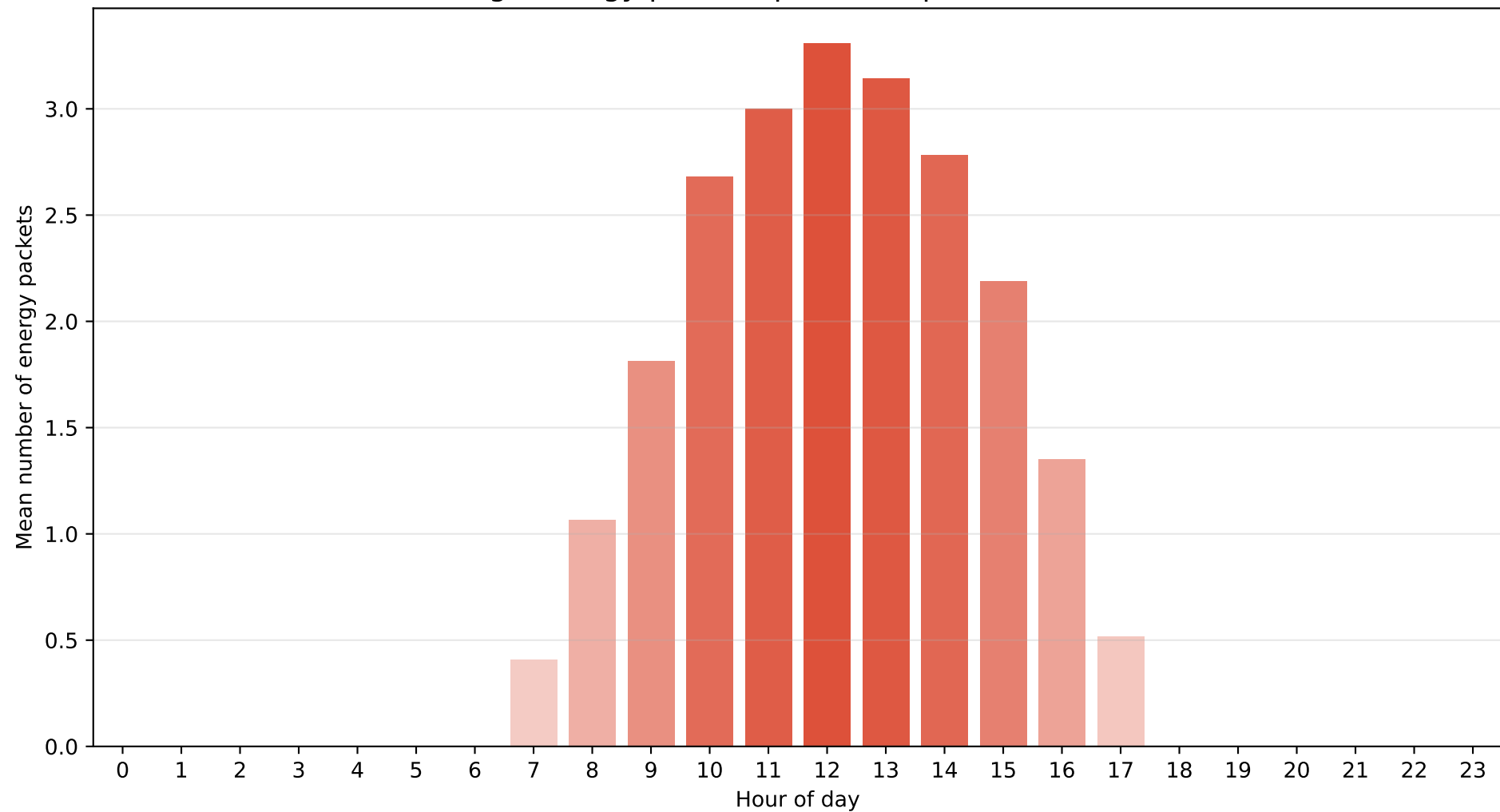
Rabat – Regime M1 (Cloudy) Average energy packets per hour (packet = 800 Wh)
