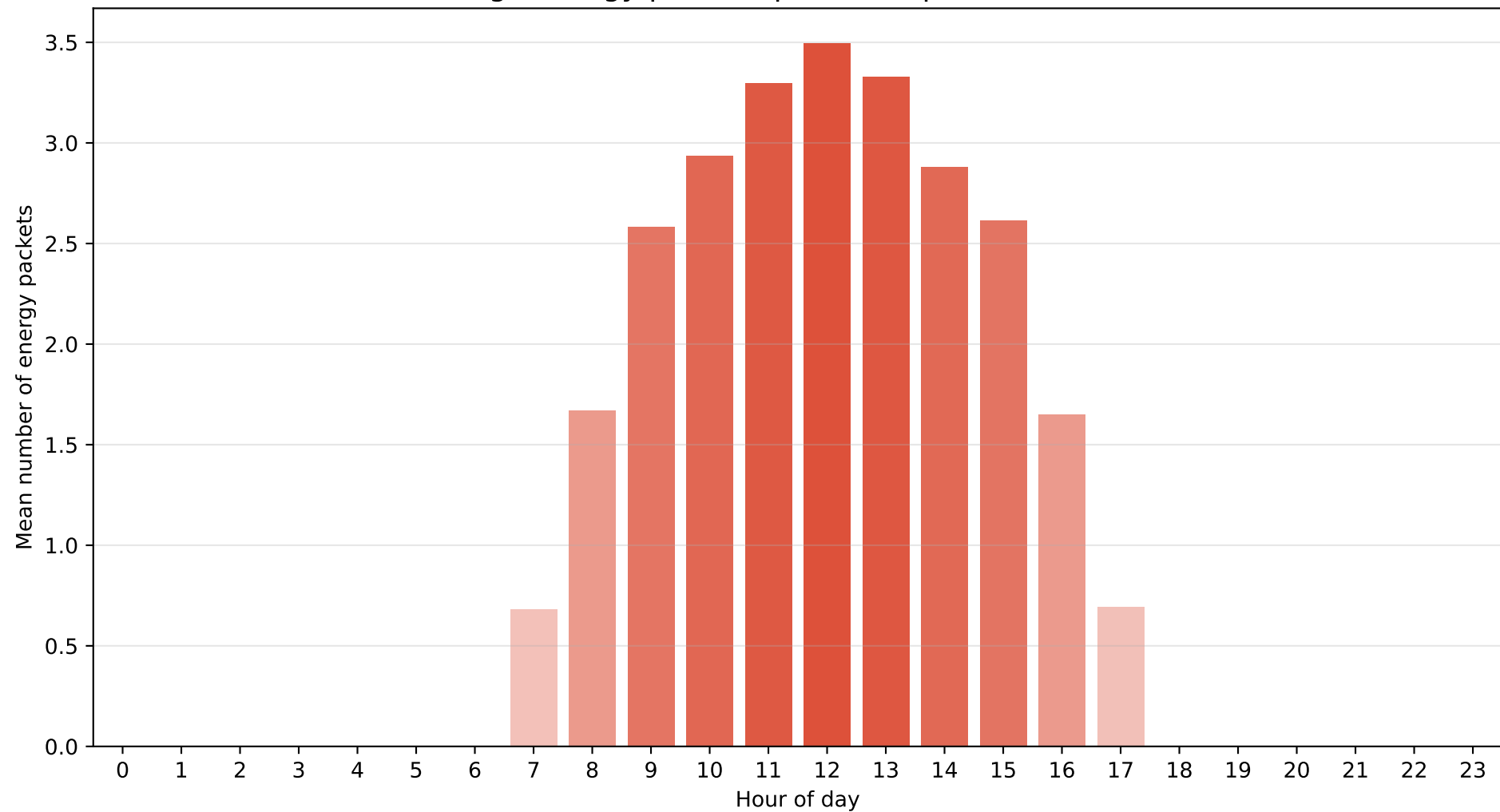
Athens – Regime M2 (Partly cloudy) Average energy packets per hour (packet = 800 Wh)
