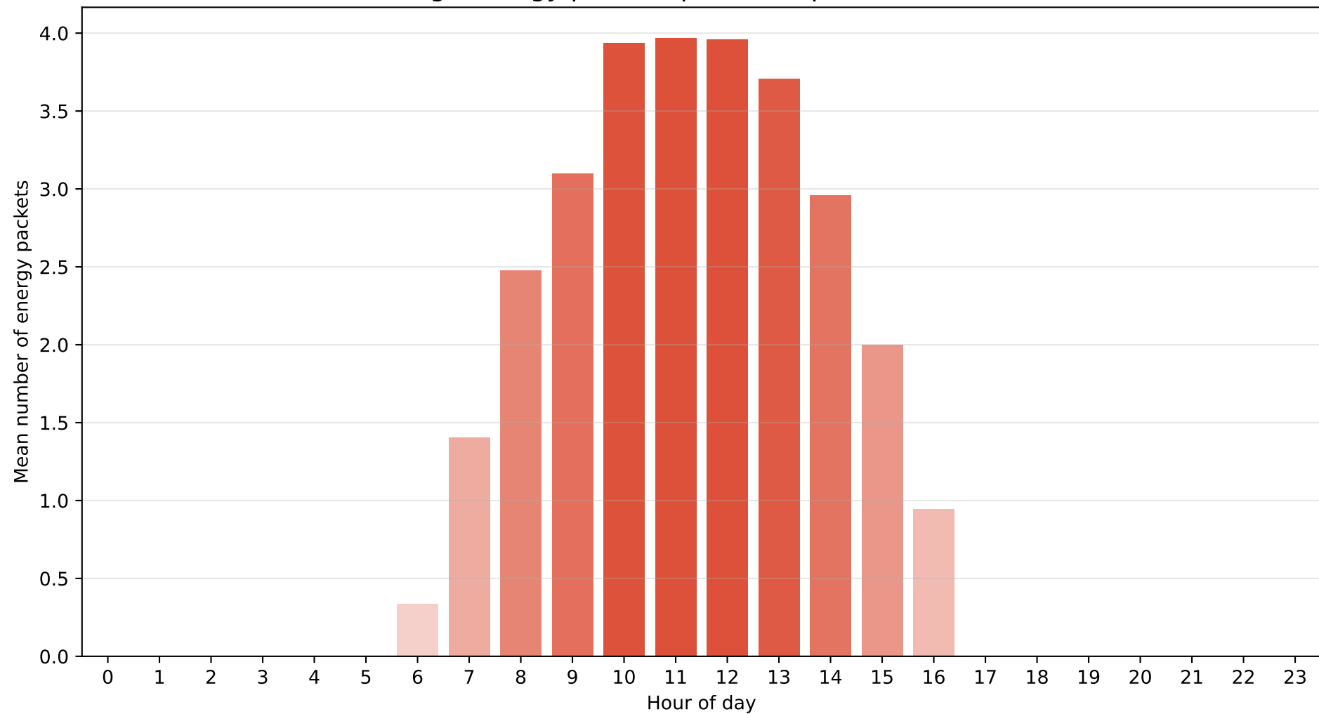
Santiago - Regime M3 (Clear sky) Average energy packets per hour (packet = 800 Wh)
