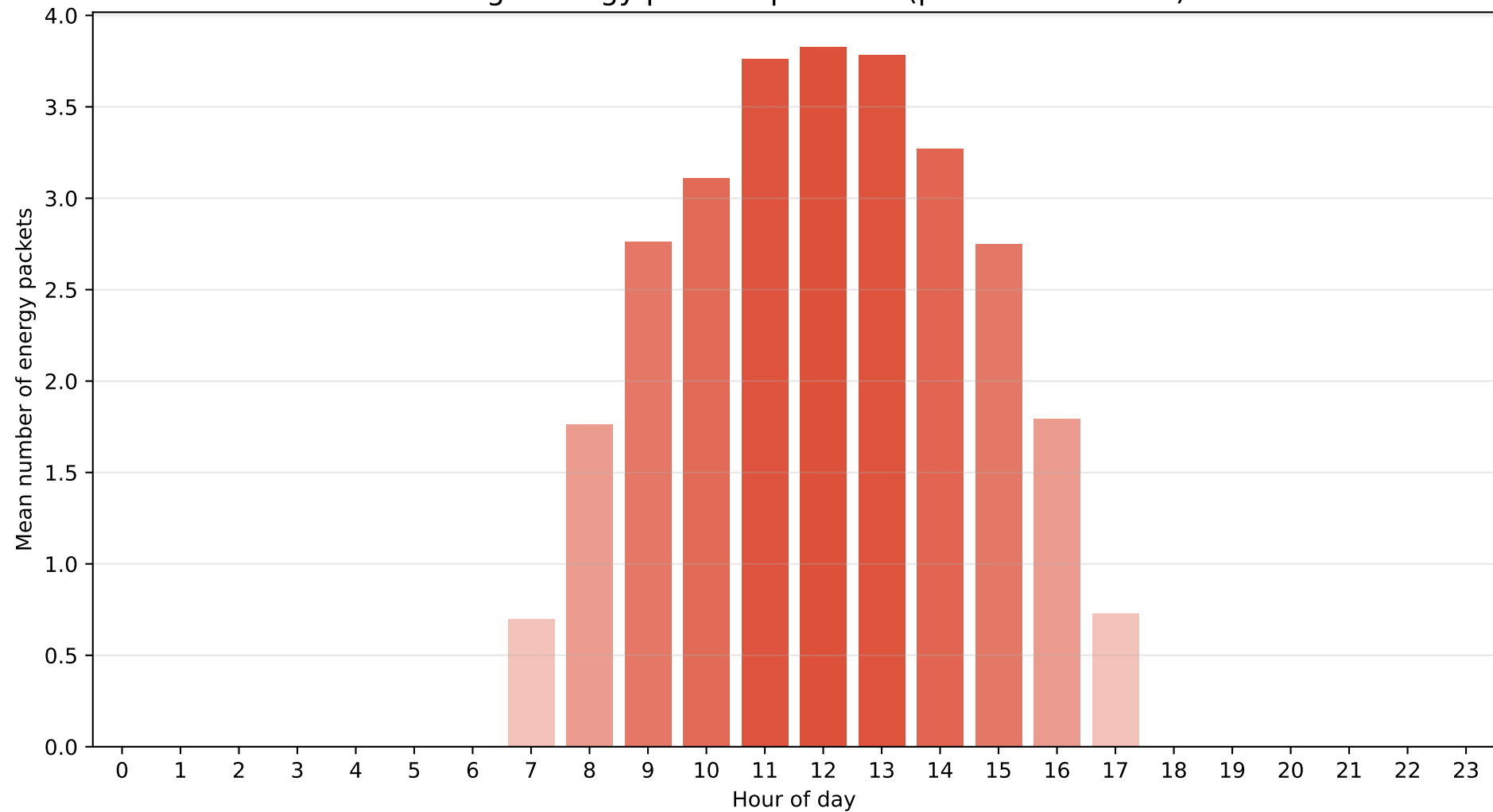
Rabat – Regime M3 (Clear sky) Average energy packets per hour (packet = 800 Wh)
