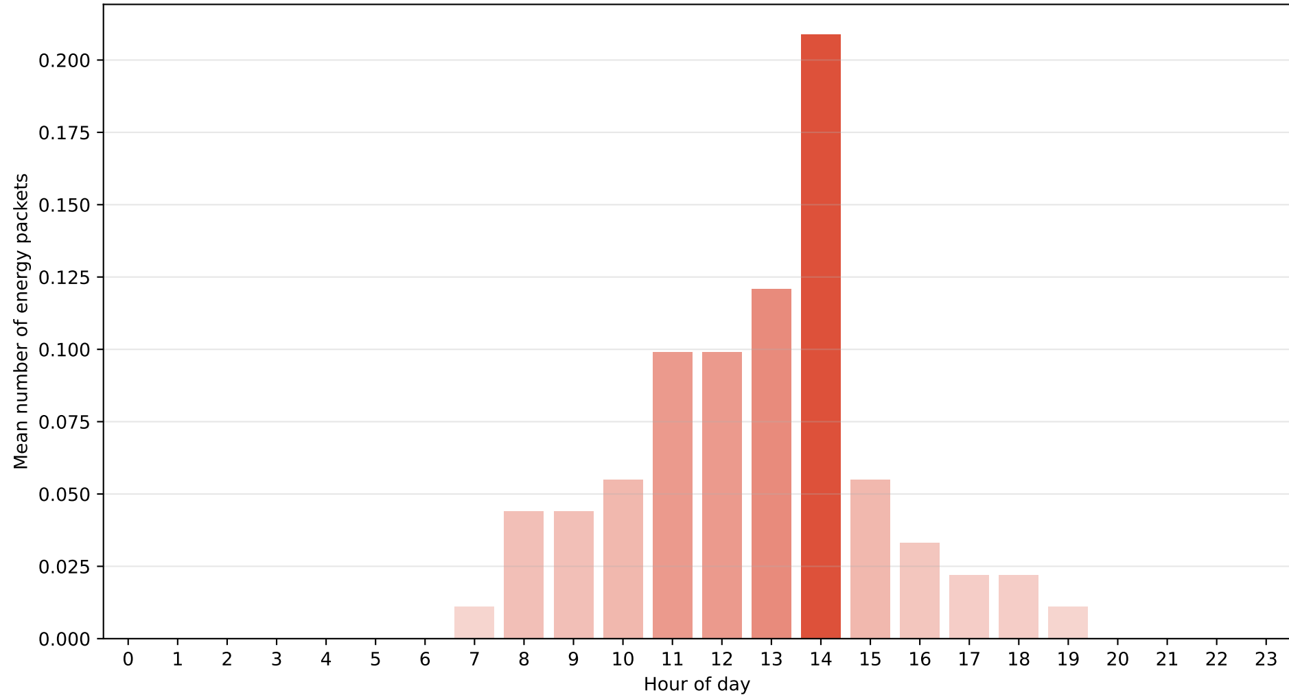
Moscow - Regime M0 (Very cloudy) Average energy packets per hour (packet = 800 Wh)
