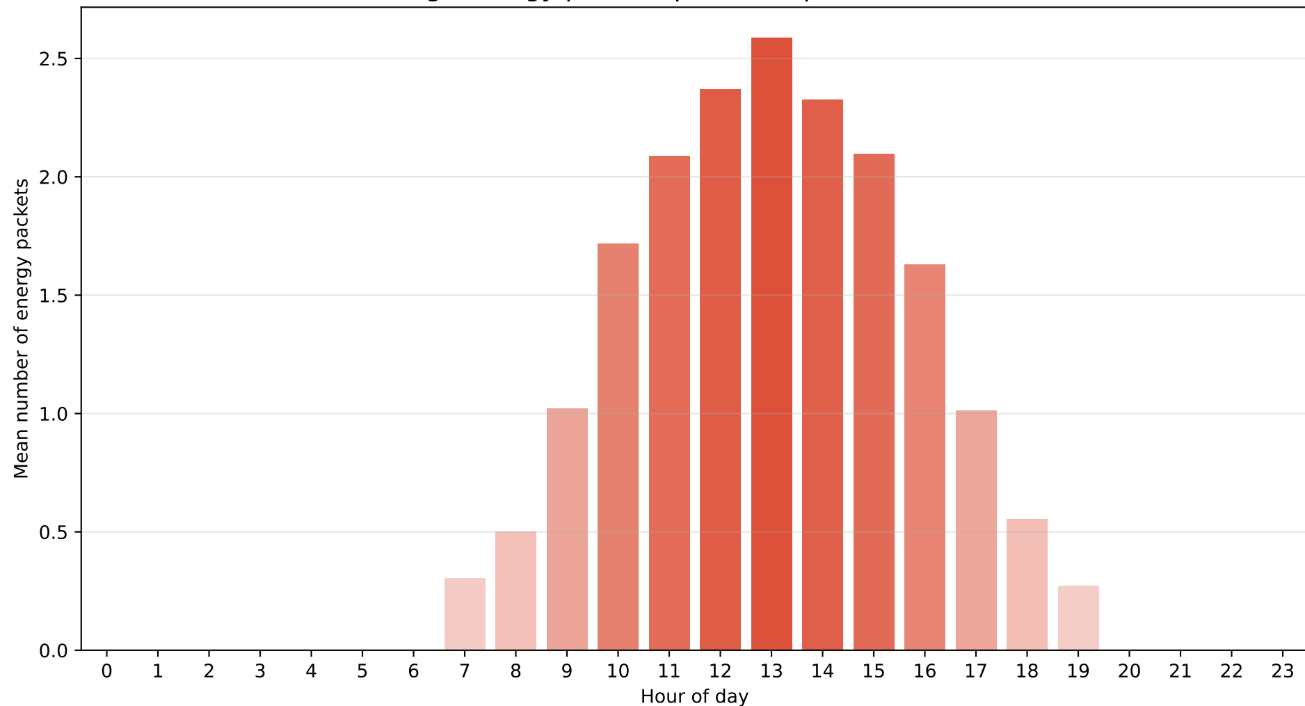
Reykjavik – Regime M3 (Clear sky) Average energy packets per hour (packet = 800 Wh)
