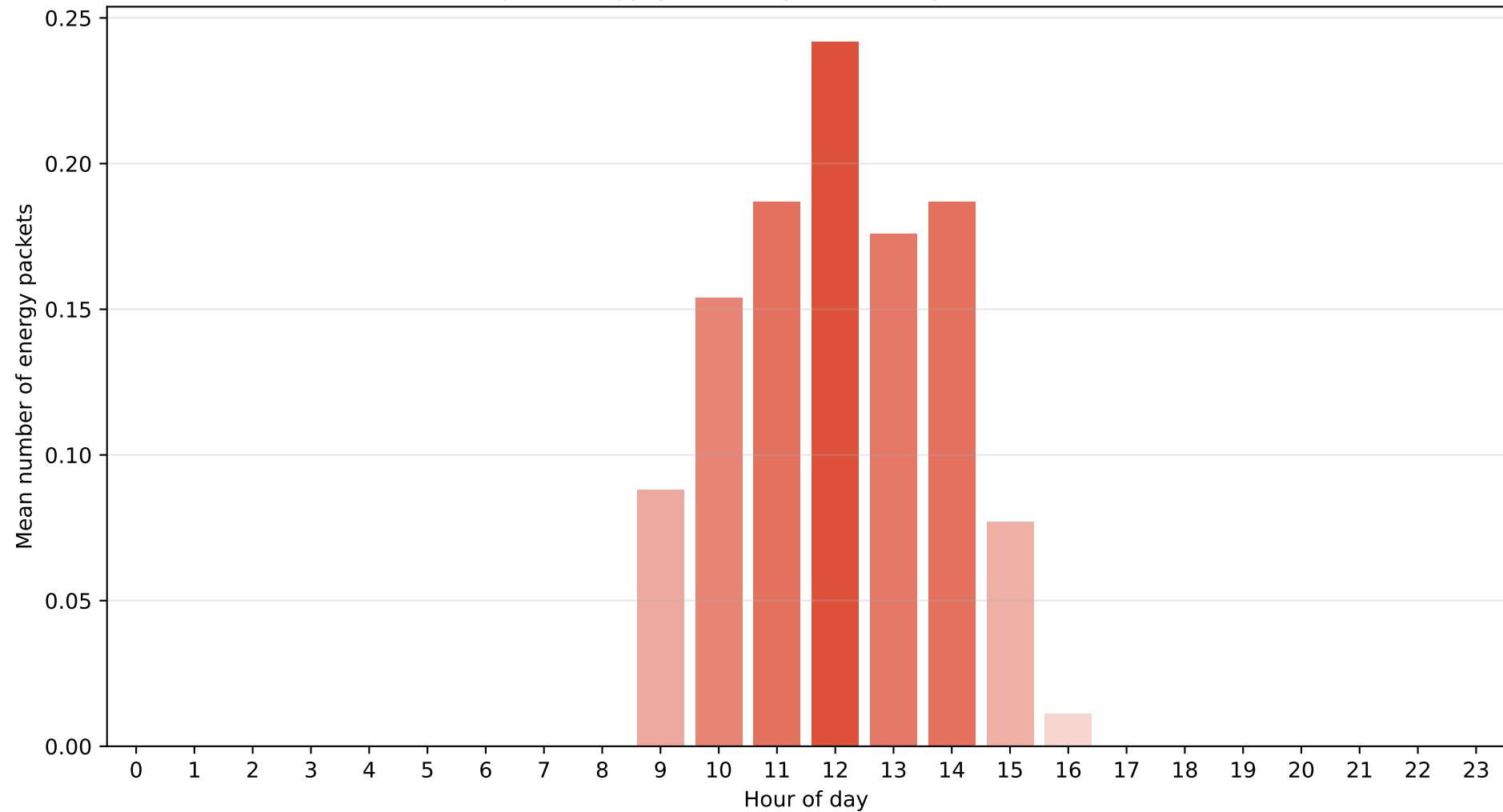
London - Regime M0 (Very cloudy) Average energy packets per hour (packet = 800 Wh)
