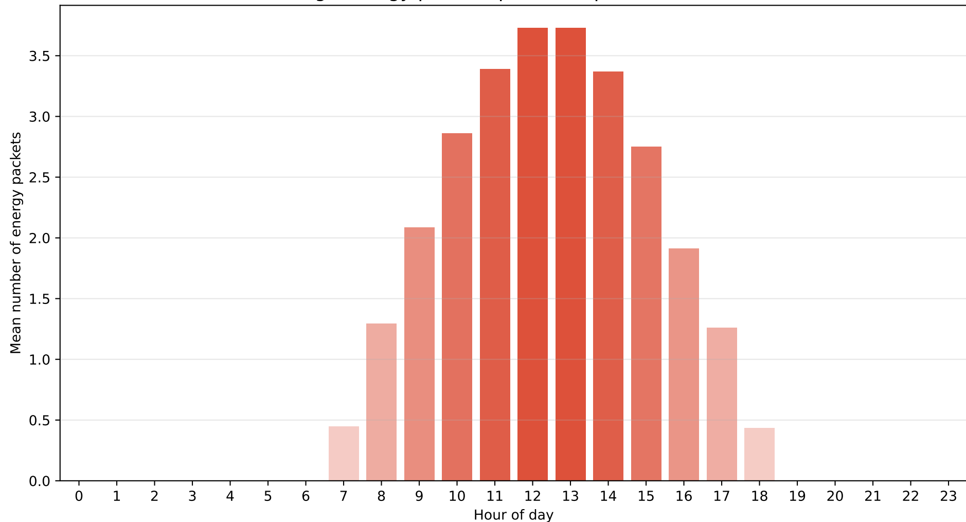
Barcelona – Regime M3 (Clear sky) Average energy packets per hour (packet = 800 Wh)
