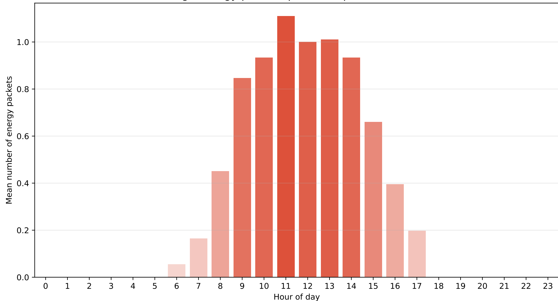
London – Regime M1 (Cloudy) Average energy packets per hour (packet = 800 Wh)
