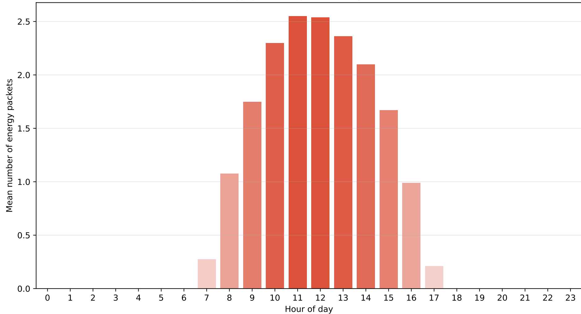
Yaounde – Regime M2 (Partly cloudy) Average energy packets per hour (packet = 800 Wh)
