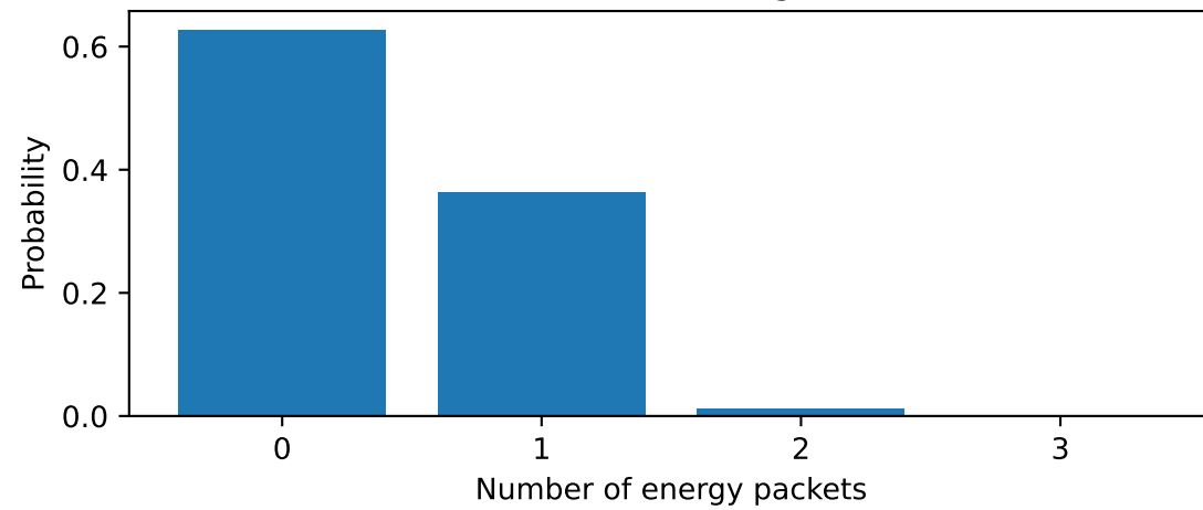
Hour 10:00 - Average 0.38
