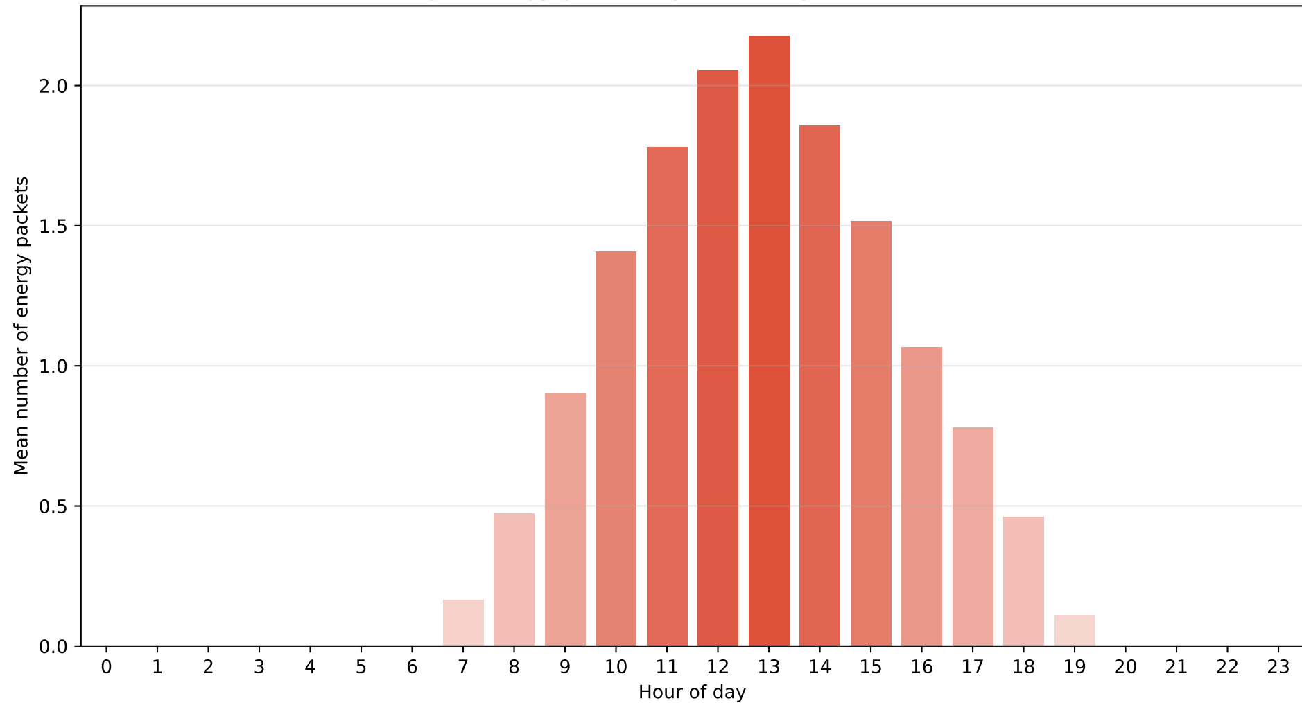
Moscow – Regime M2 (Partly cloudy) Average energy packets per hour (packet = 800 Wh)
