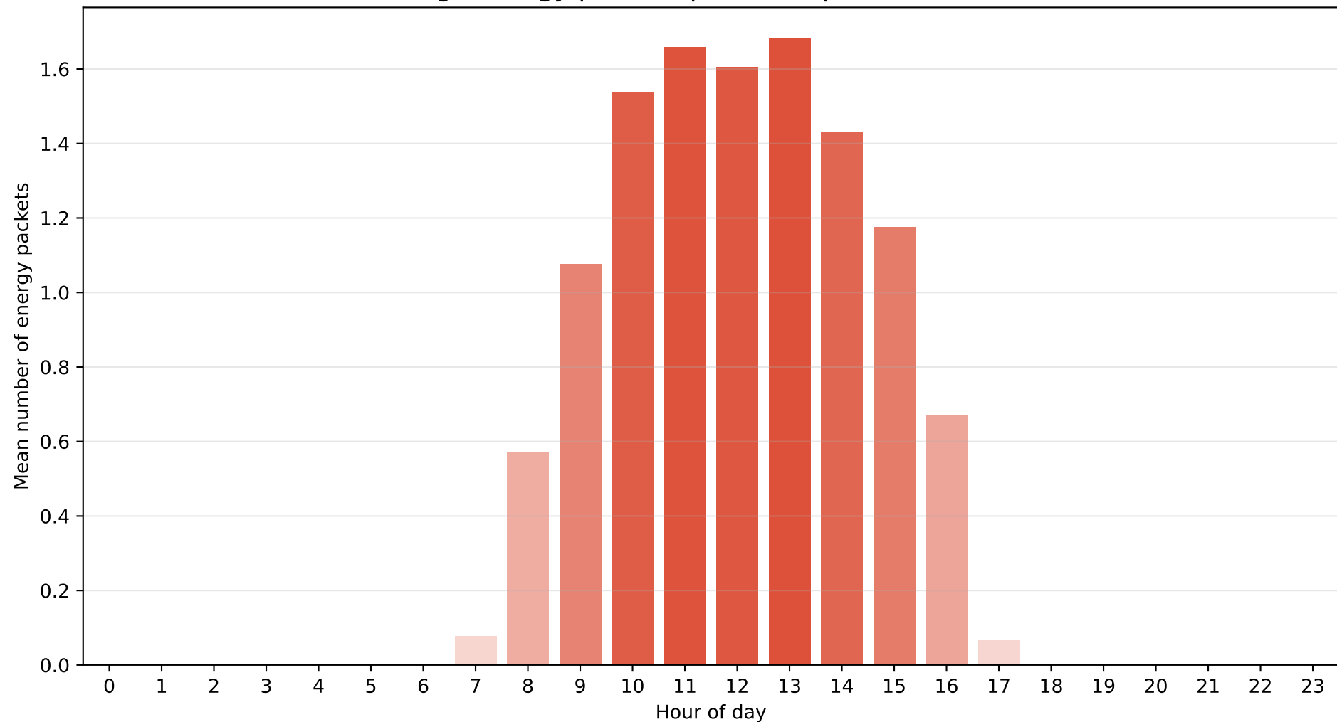
Yaounde – Regime M0 (Very cloudy) Average energy packets per hour (packet = 800 Wh)
