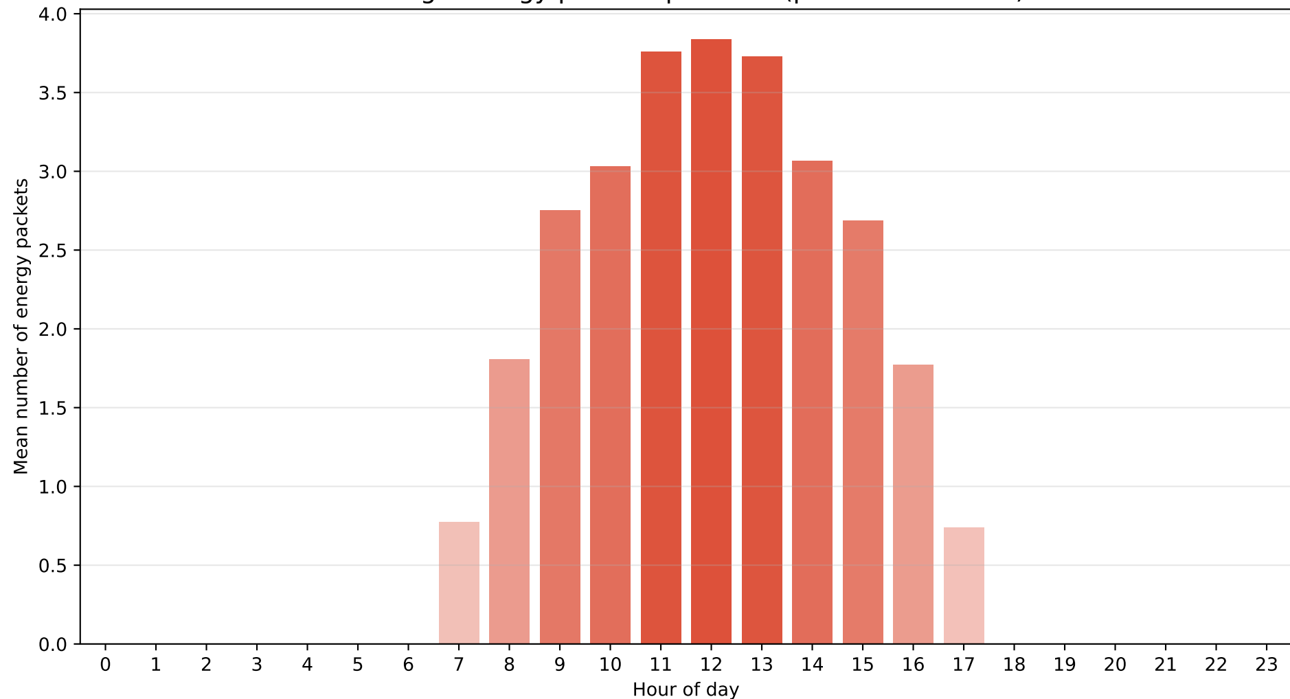
Athens - Regime M3 (Clear sky) Average energy packets per hour (packet = 800 Wh)
