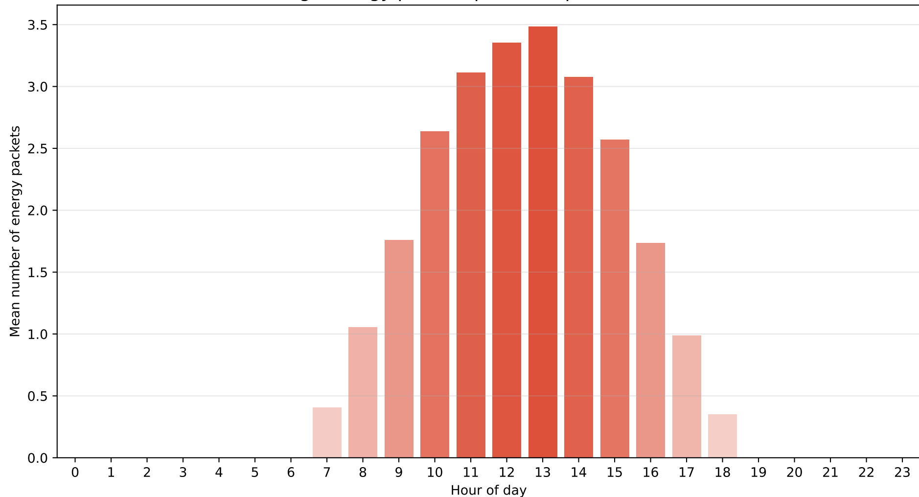
Barcelona – Regime M2 (Partly cloudy) Average energy packets per hour (packet = 800 Wh)
