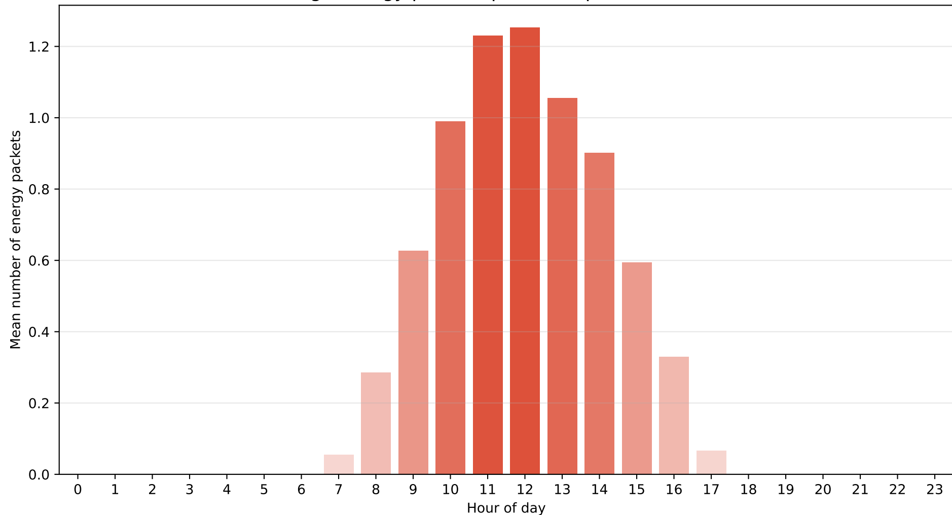
Athens – Regime M0 (Very cloudy) Average energy packets per hour (packet = 800 Wh)
