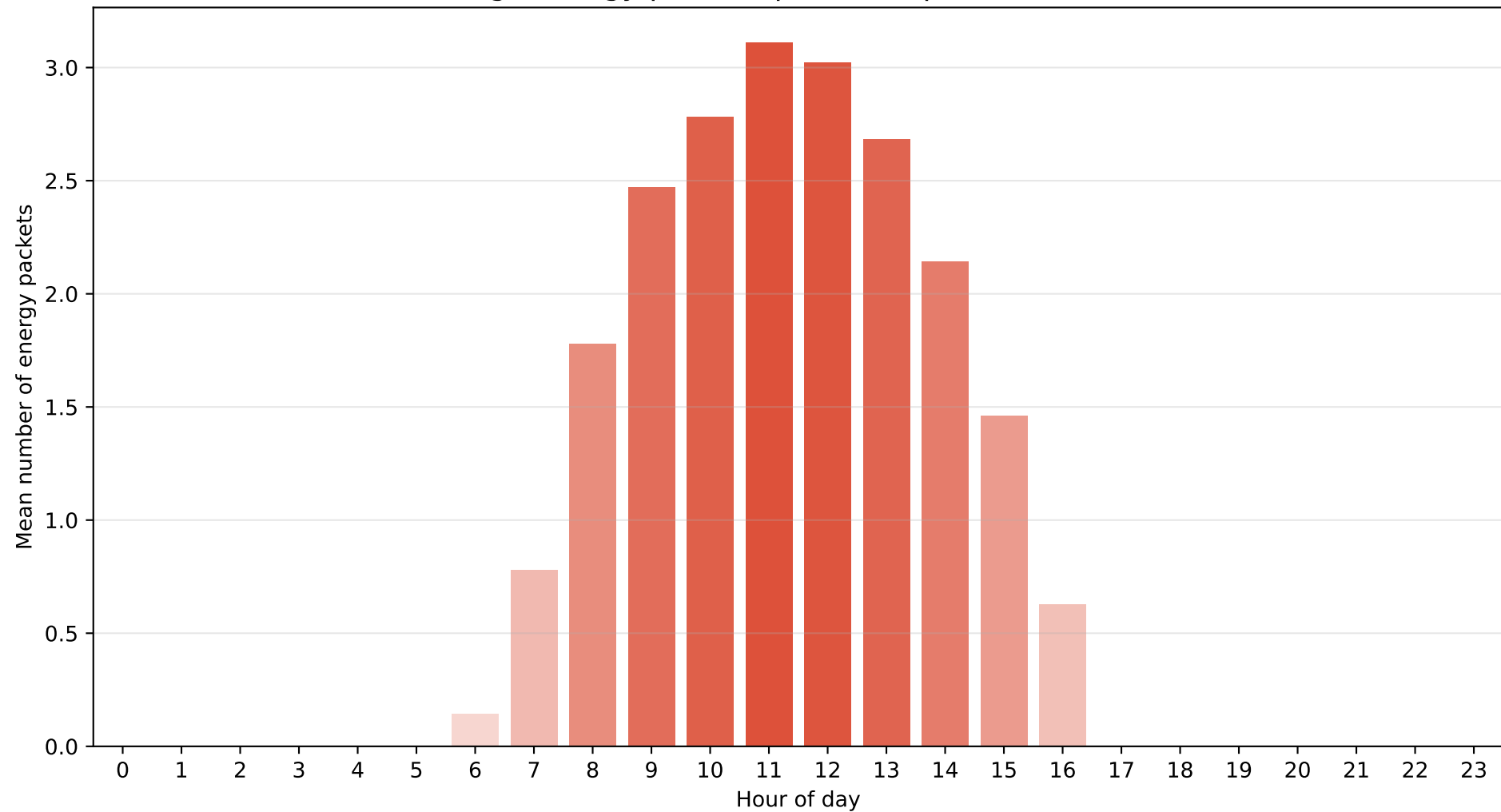
Santiago – Regime M1 (Cloudy) Average energy packets per hour (packet = 800 Wh)
