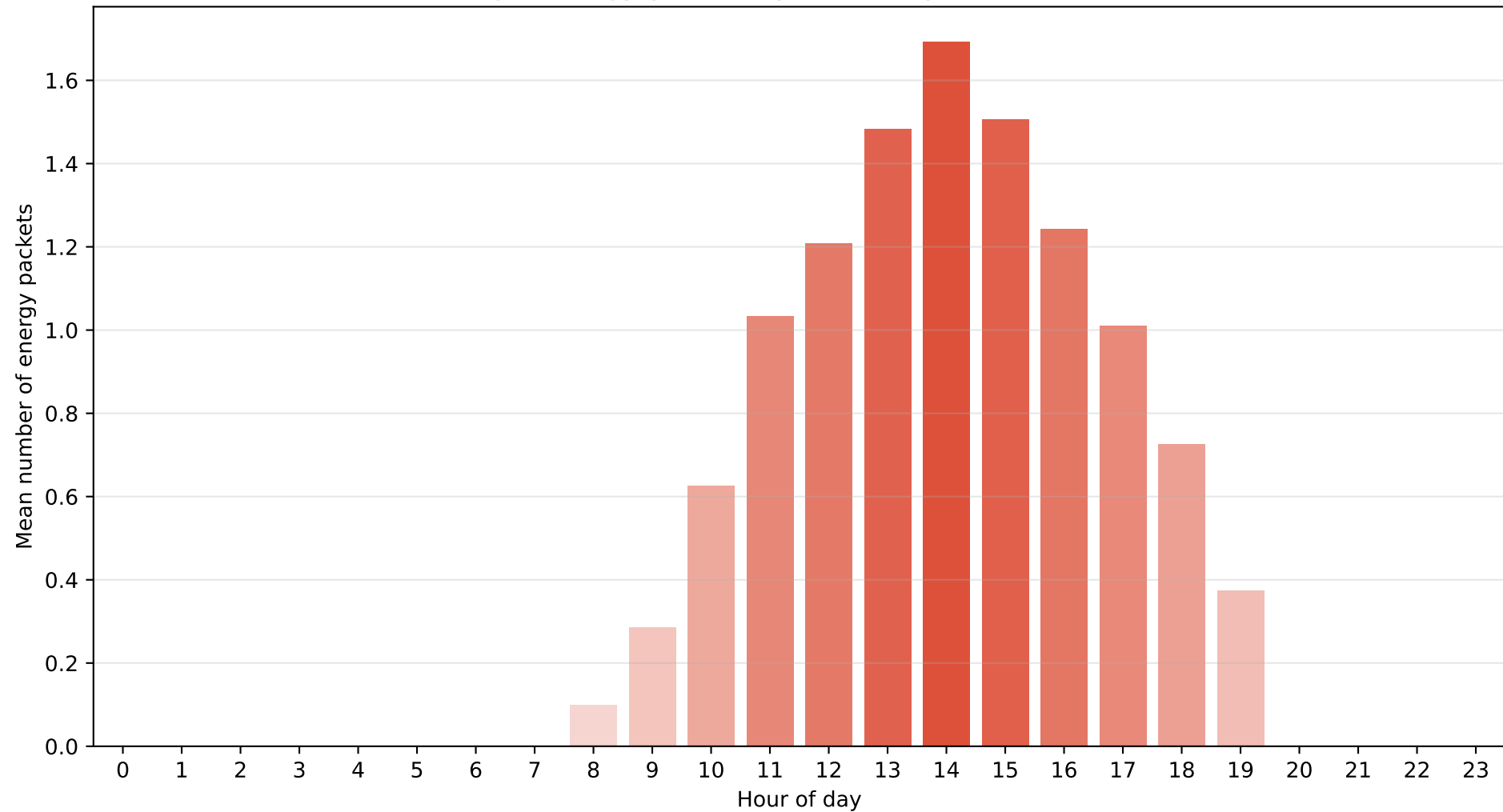
Unalaska - Regime M2 (Partly cloudy) Average energy packets per hour (packet = 800 Wh)
