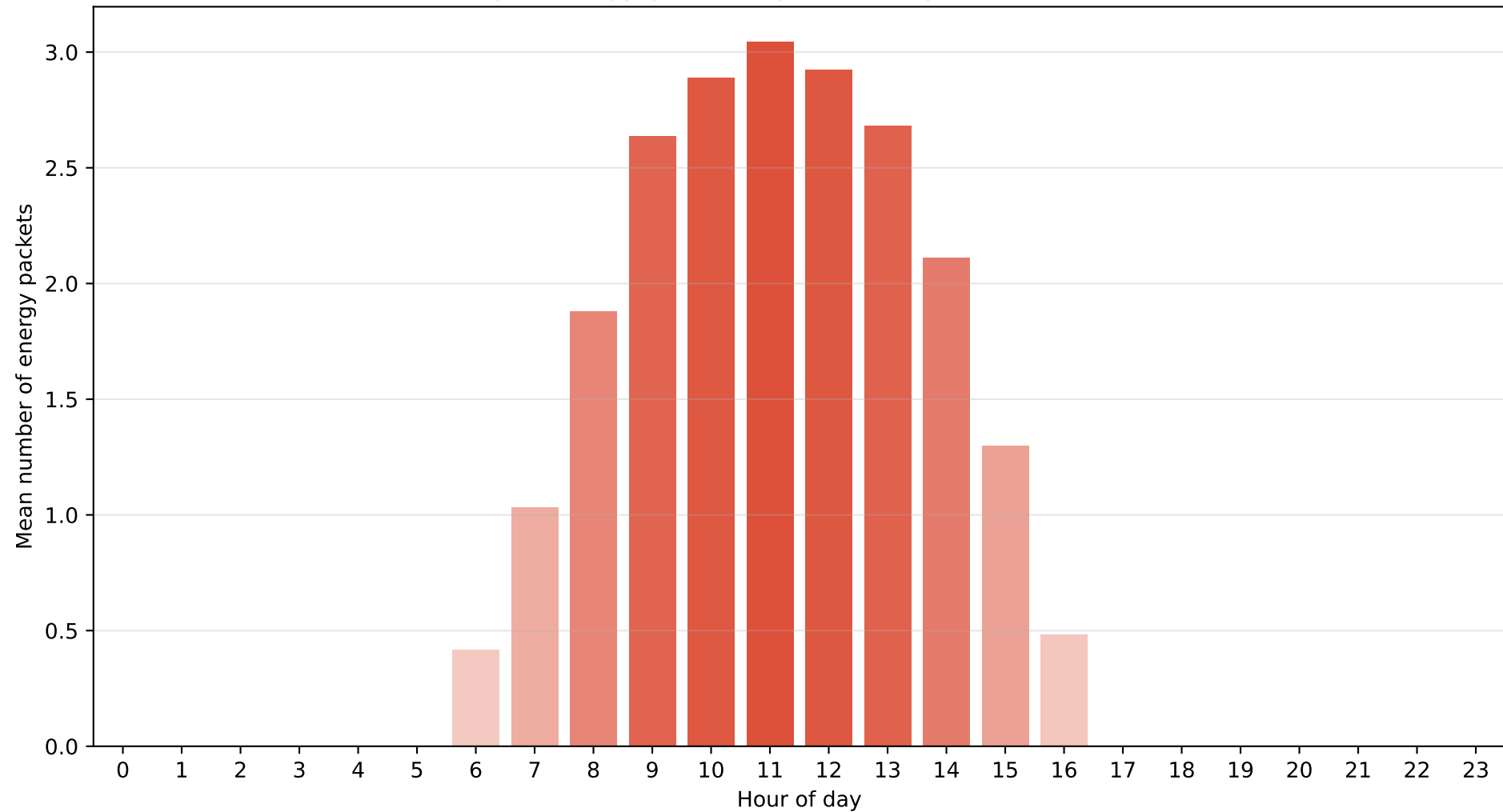
Tokyo - Regime M2 (Partly cloudy) Average energy packets per hour (packet = 800 Wh)
