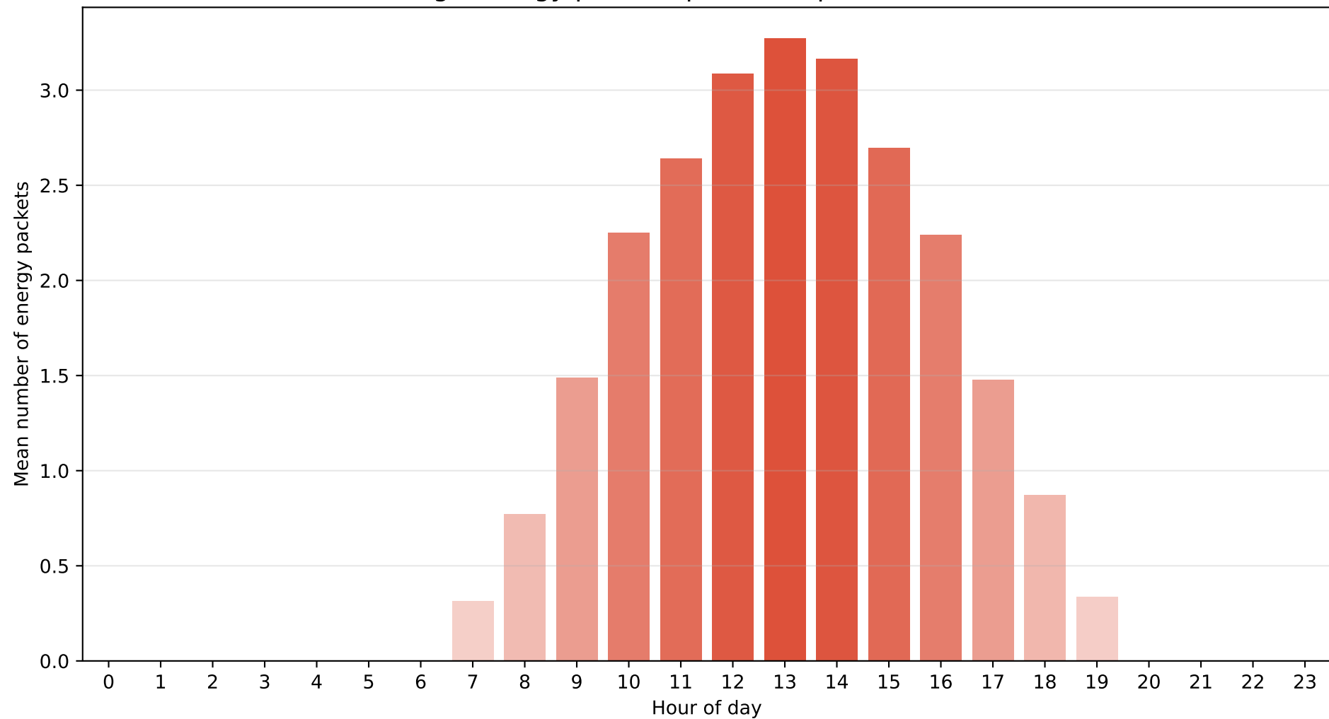
Moscow – Regime M3 (Clear sky) Average energy packets per hour (packet = 800 Wh)
