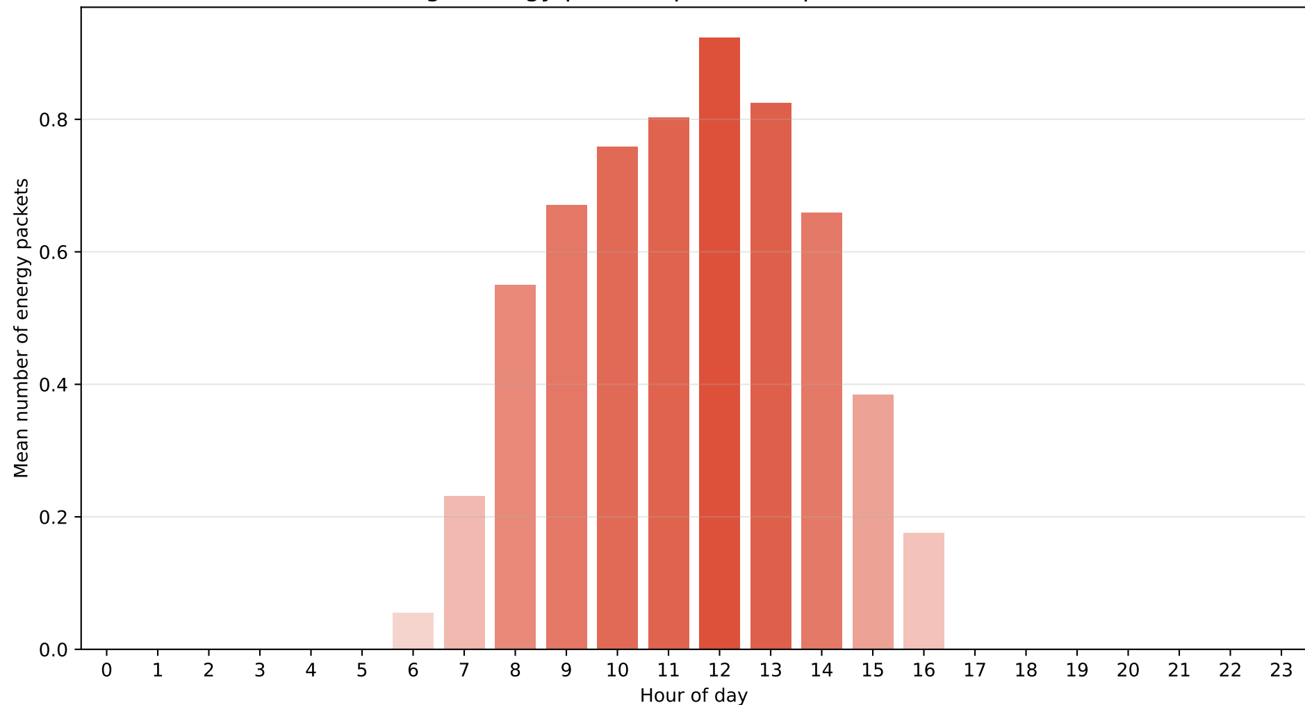
Tokyo – Regime M0 (Very cloudy) Average energy packets per hour (packet = 800 Wh)
