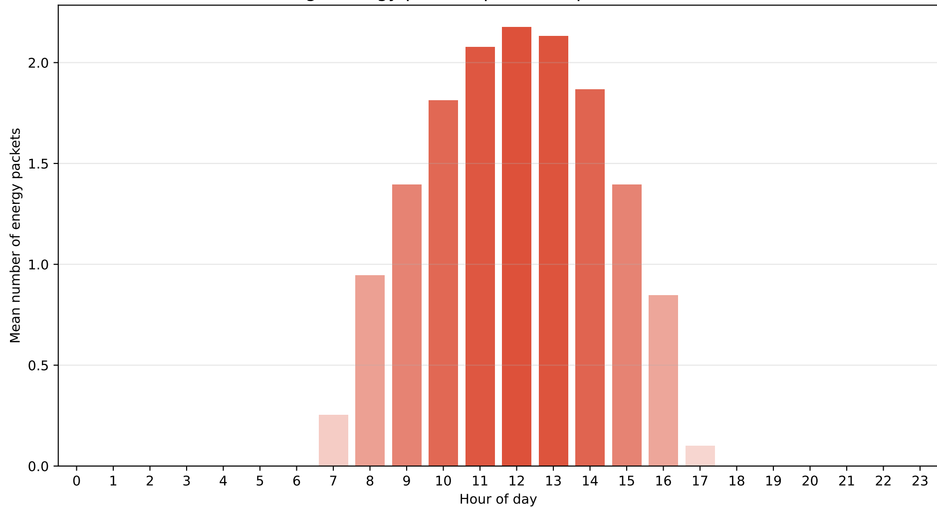
Yaounde - Regime M1 (Cloudy) Average energy packets per hour (packet = 800 Wh)
