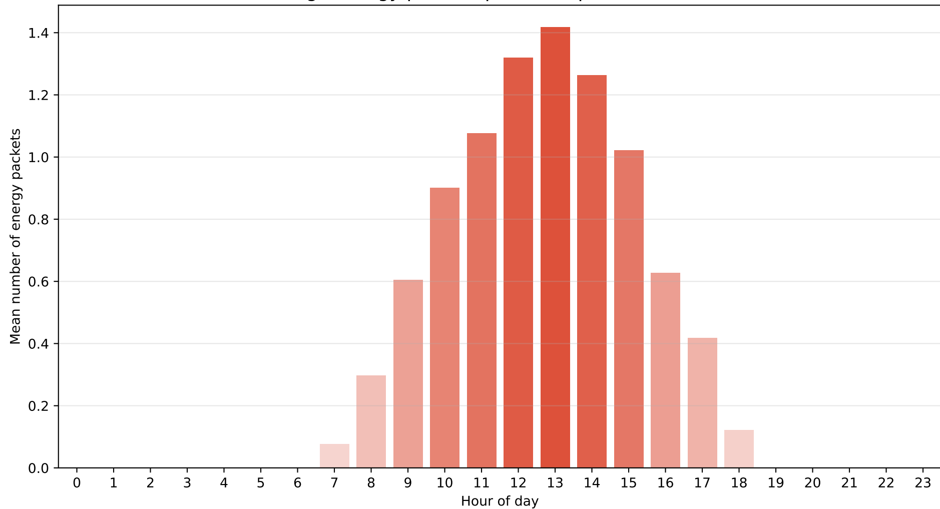
Paris - Regime M1 (Cloudy) Average energy packets per hour (packet = 800 Wh)
