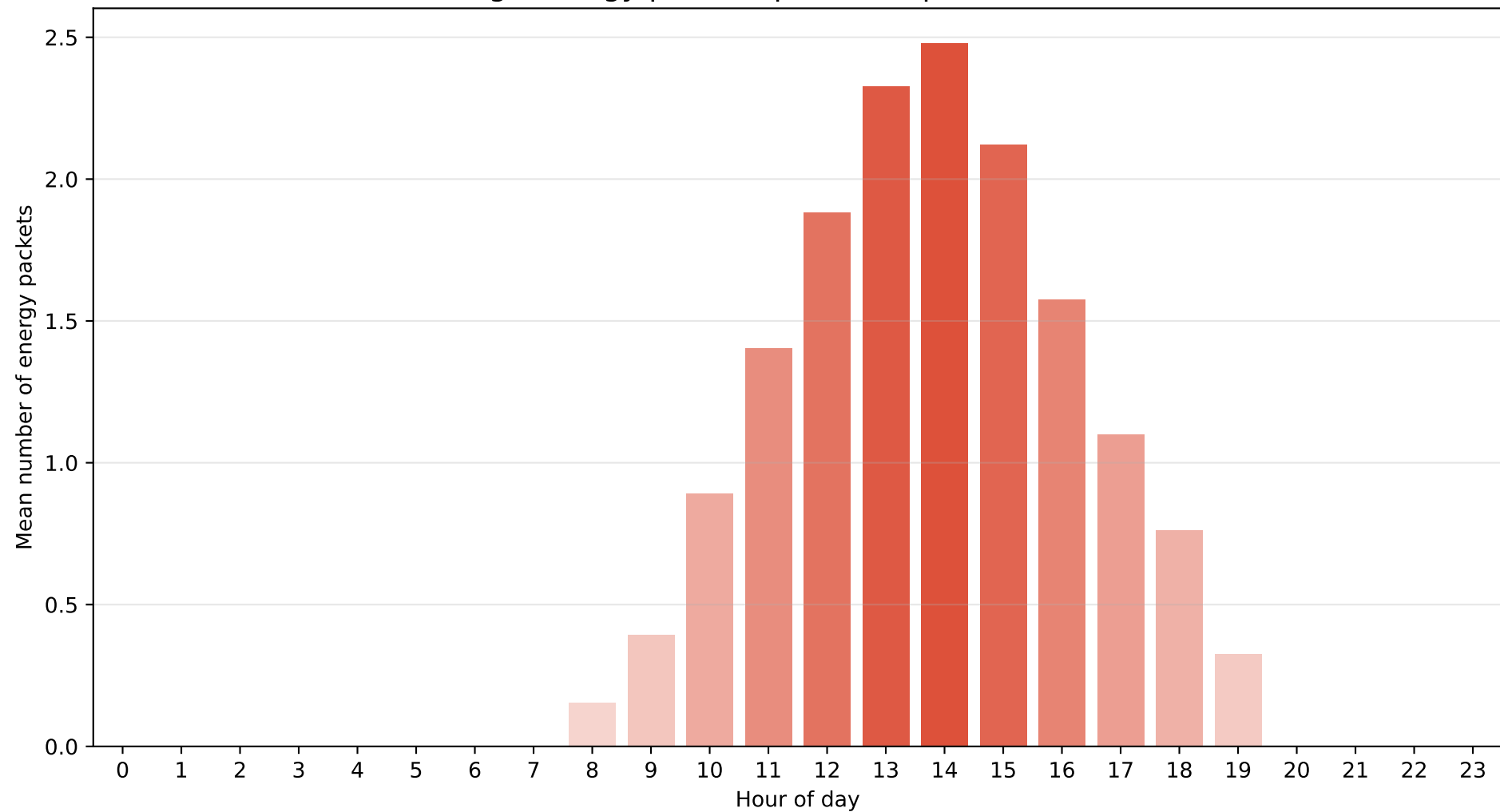
Unalaska - Regime M3 (Clear sky) Average energy packets per hour (packet = 800 Wh)
