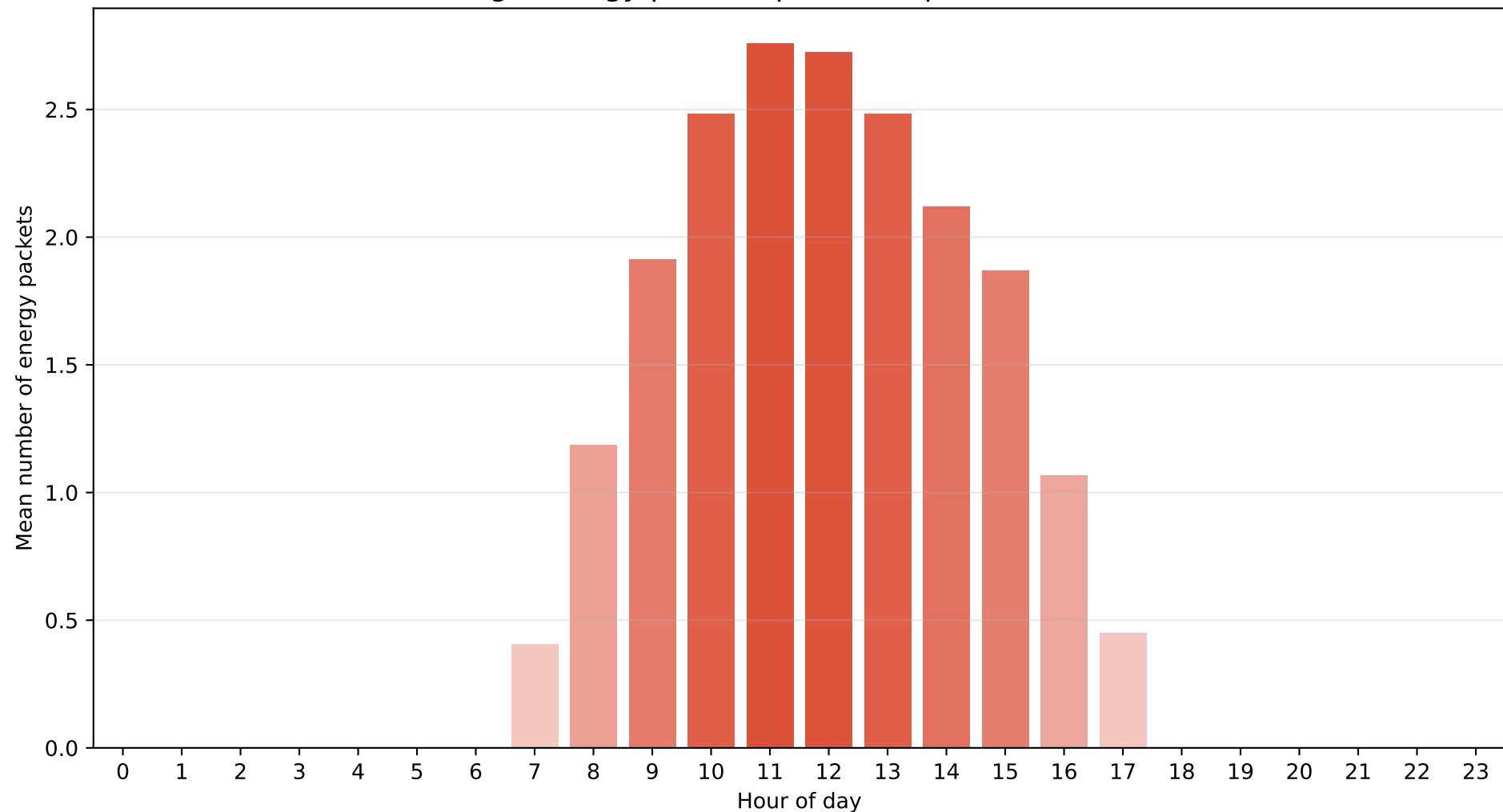
Athens – Regime M1 (Cloudy) Average energy packets per hour (packet = 800 Wh)
