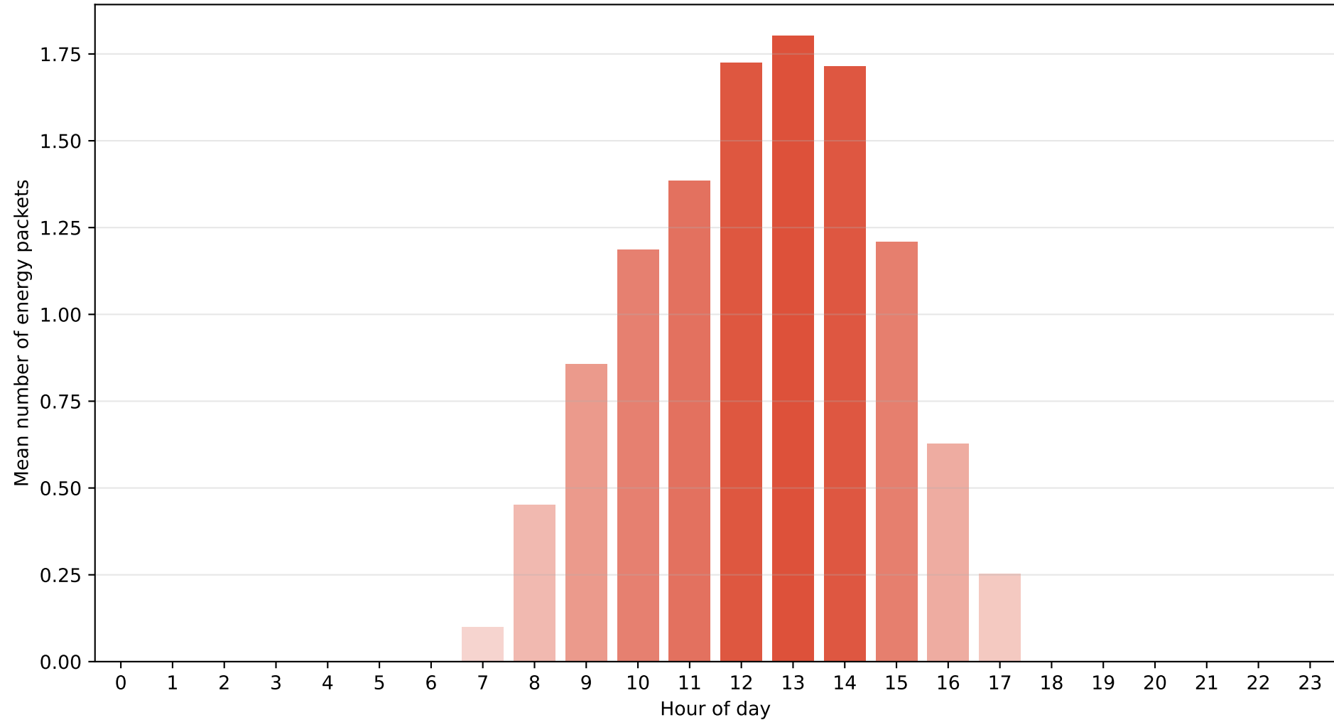
Rabat – Regime M0 (Very cloudy) Average energy packets per hour (packet = 800 Wh)
