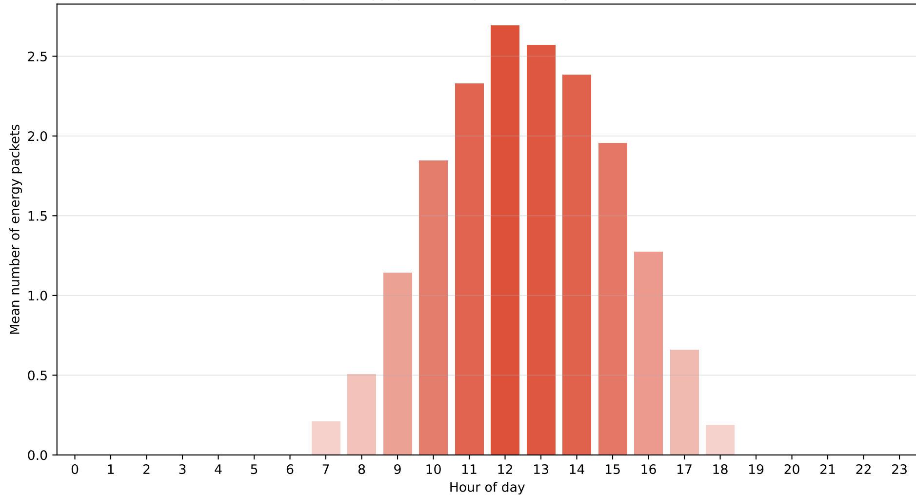
Barcelona – Regime M1 (Cloudy) Average energy packets per hour (packet = 800 Wh)
