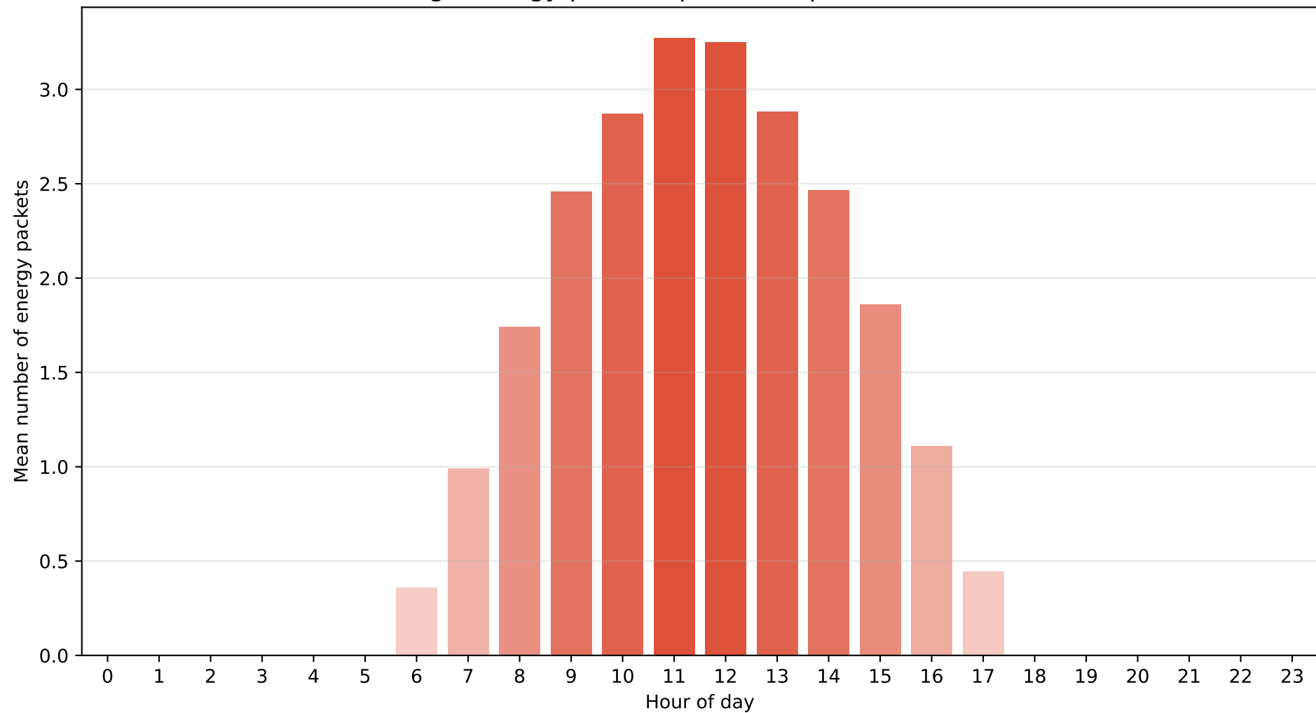
London - Regime M3 (Clear sky) Average energy packets per hour (packet = 800 Wh)
