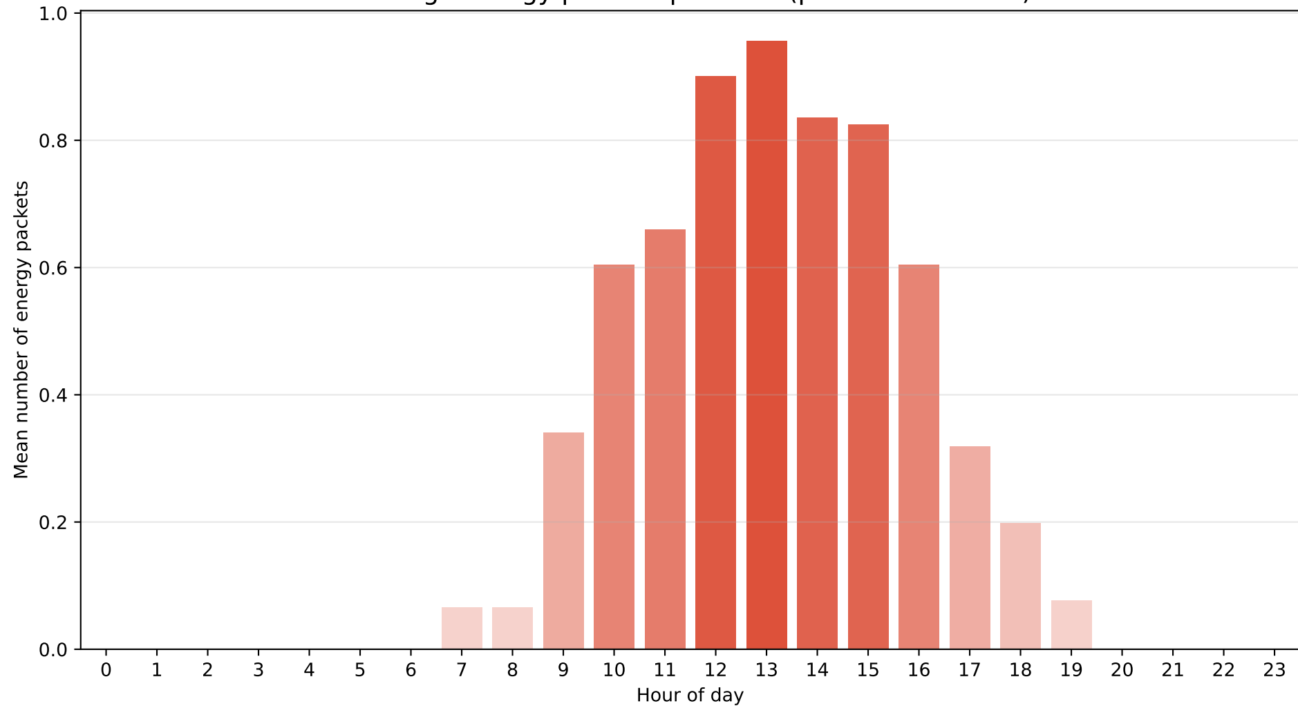
Reykjavik - Regime M1 (Cloudy) Average energy packets per hour (packet = 800 Wh)
