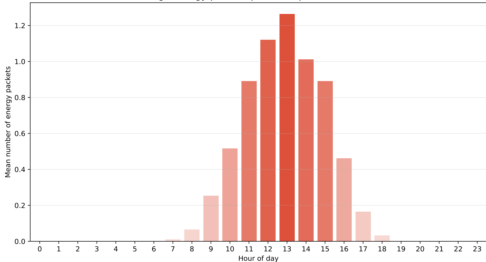
Barcelona - Regime M0 (Very cloudy) Average energy packets per hour (packet = 800 Wh)
