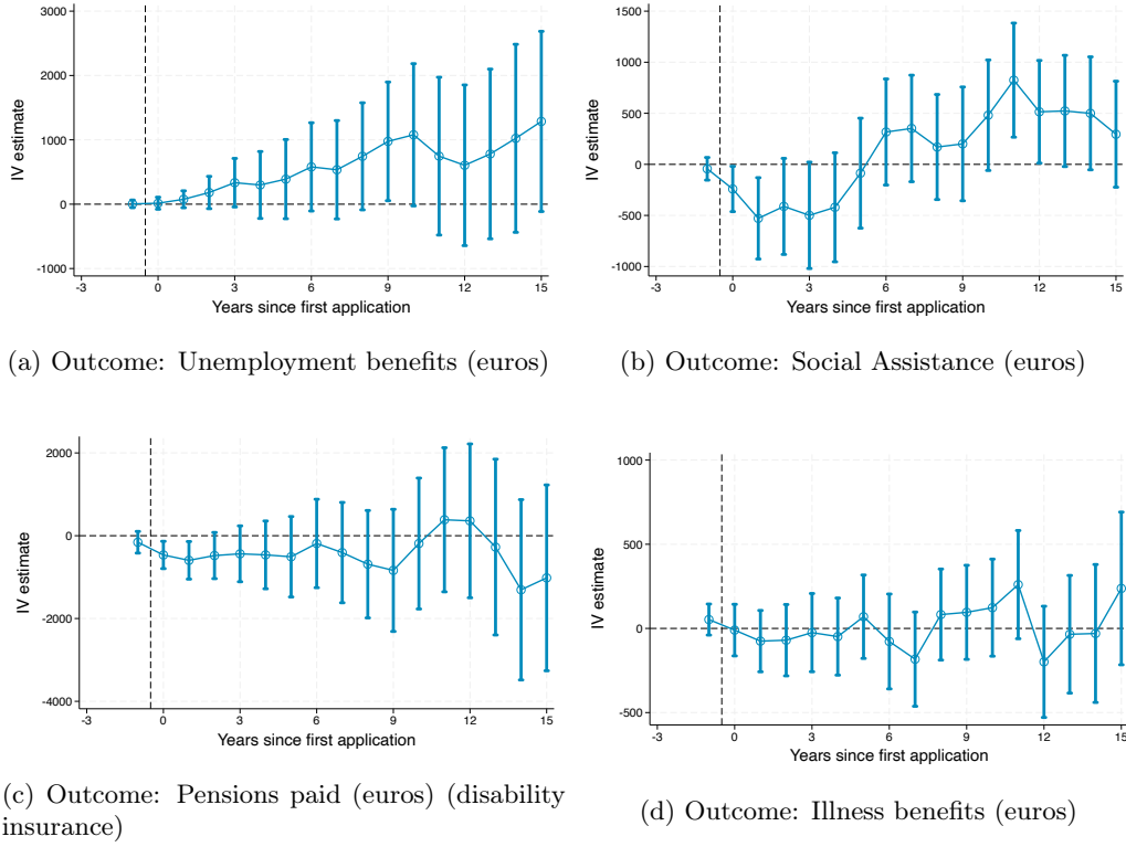
Figure A.3: Long-run (EB) IV estimates on benefits paid to individuals. Each estimate represents an IV-estimate from a separate regression using time-specific samples. Outcomes apart from health are not necessarily informative for individuals younger than 16 years old, which moves pre-treatment estimates toward 0.
