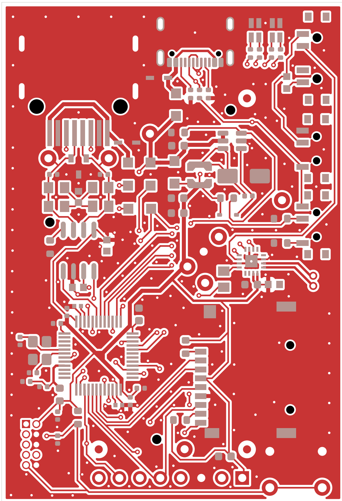
Figure 1.2: UACS PCB — front copper layer (F.Cu).
