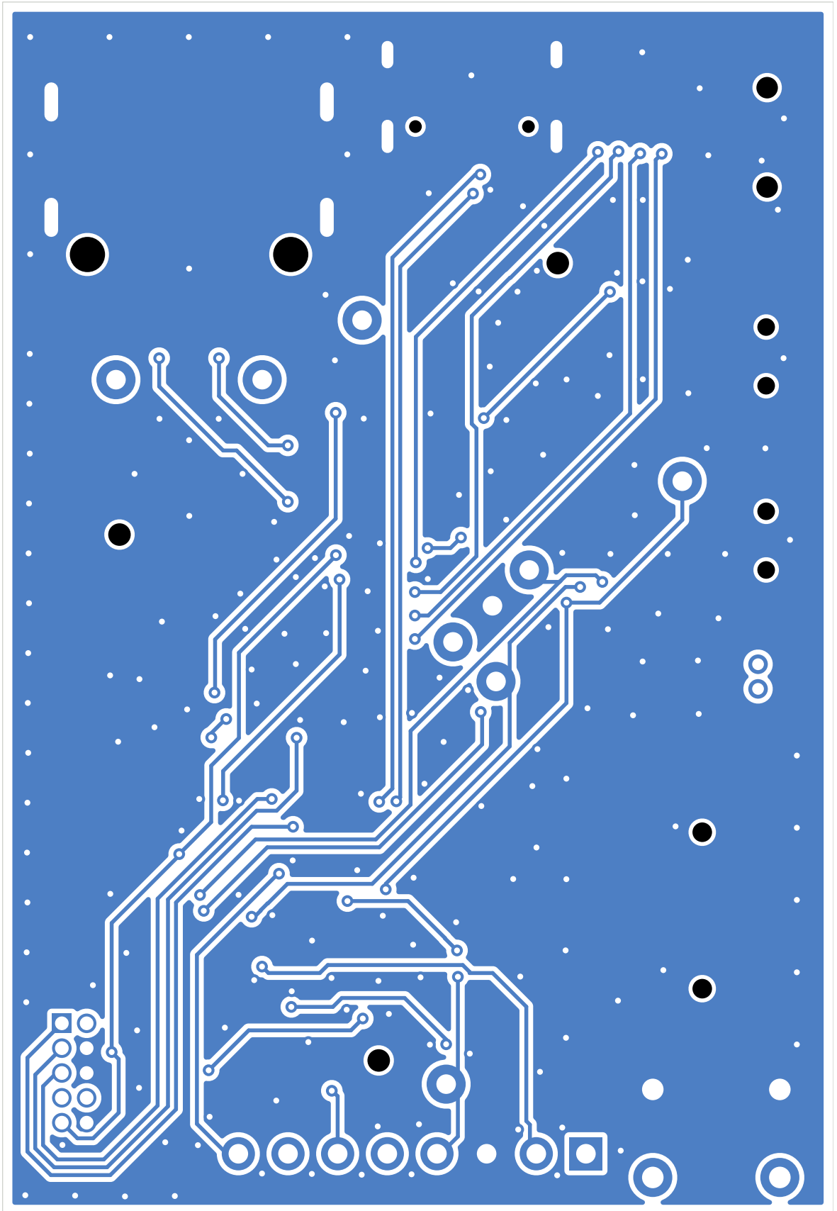
Figure 1.3: UACS PCB — back copper layer (B.Cu).
