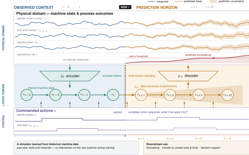
Figure 2: A CNC world model in practice. The schematic illustrates the operational interpretation of the learned dynamics model. Recent sensor measurements are encoded into a latent state, future control actions condition multi-horizon latent predictions, and a physical decoder maps predicted latent states to multi-horizon process variables and uncertainty. The figure is conceptual and does not constitute a closed-loop deployment result. Its purpose is to distinguish passive forecasting from action-conditioned simulation of candidate futures. The chain of latent states and the operational-risk lane are illustrative: the implementation predicts all horizons in one pass from the context latent (Sec. 4.2), and the risk variable is a downstream use, not an output of the model in this paper.
