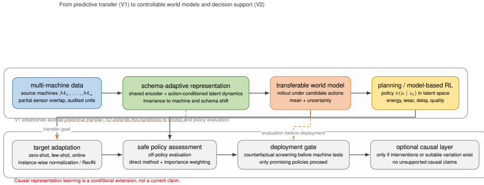
Figure 7: V1 establishes audited cross-machine predictive transfer with schema-adaptive latent dynamics. V2 extends this backbone to multi-machine representation learning, target adaptation with stronger normalization, action-conditioned planning or model-based RL, and policy assessment through off-policy evaluation before any physical deployment. Optional causal representation learning is shown as a conditional branch rather than as a current contribution.
