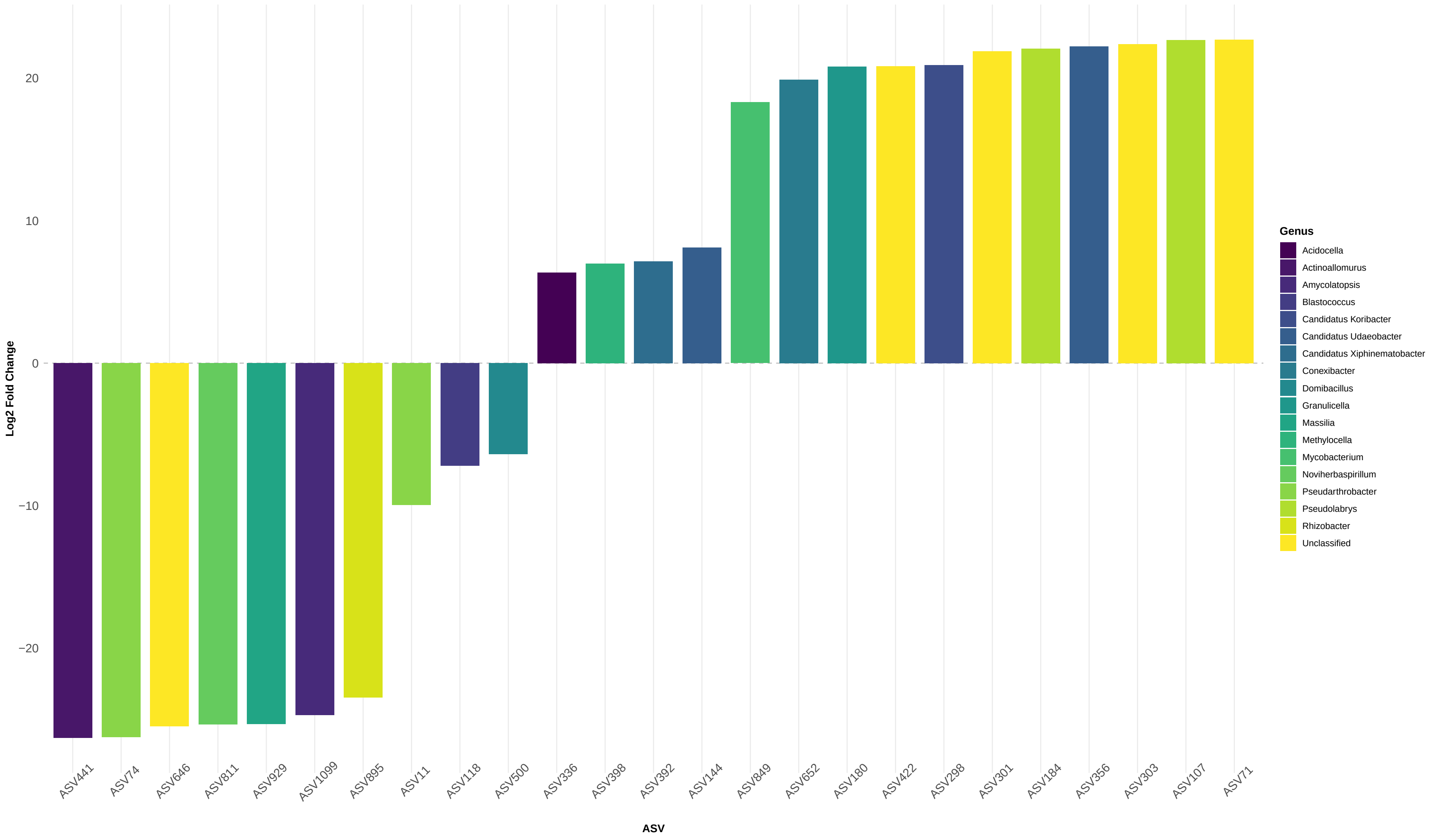
Differential Abundance Analysis: Fire_Mod_untreated_vs_wildfire
