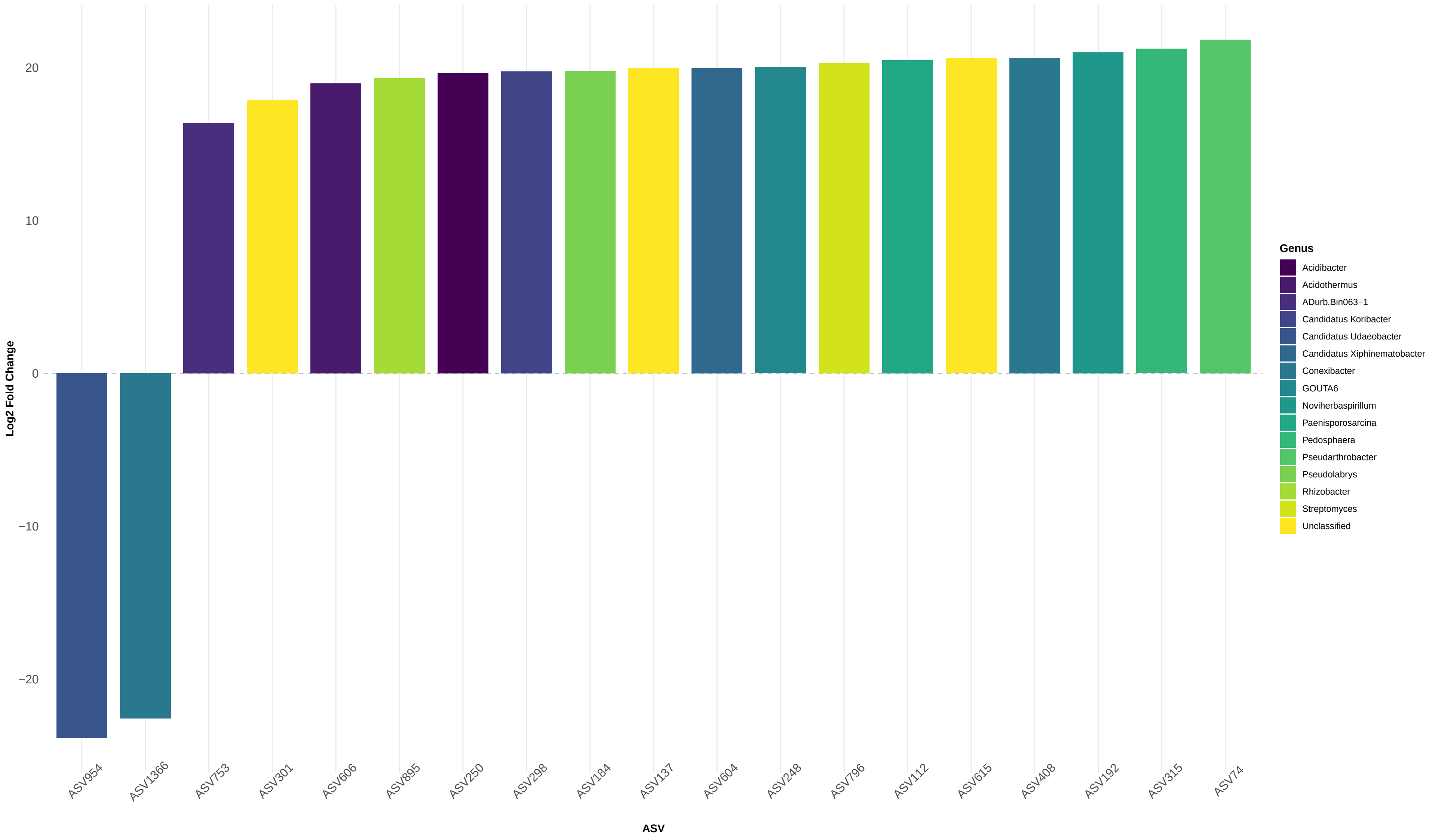
Differential Abundance Analysis: YrSinceTrt_BR_1to2_vs_5to8
