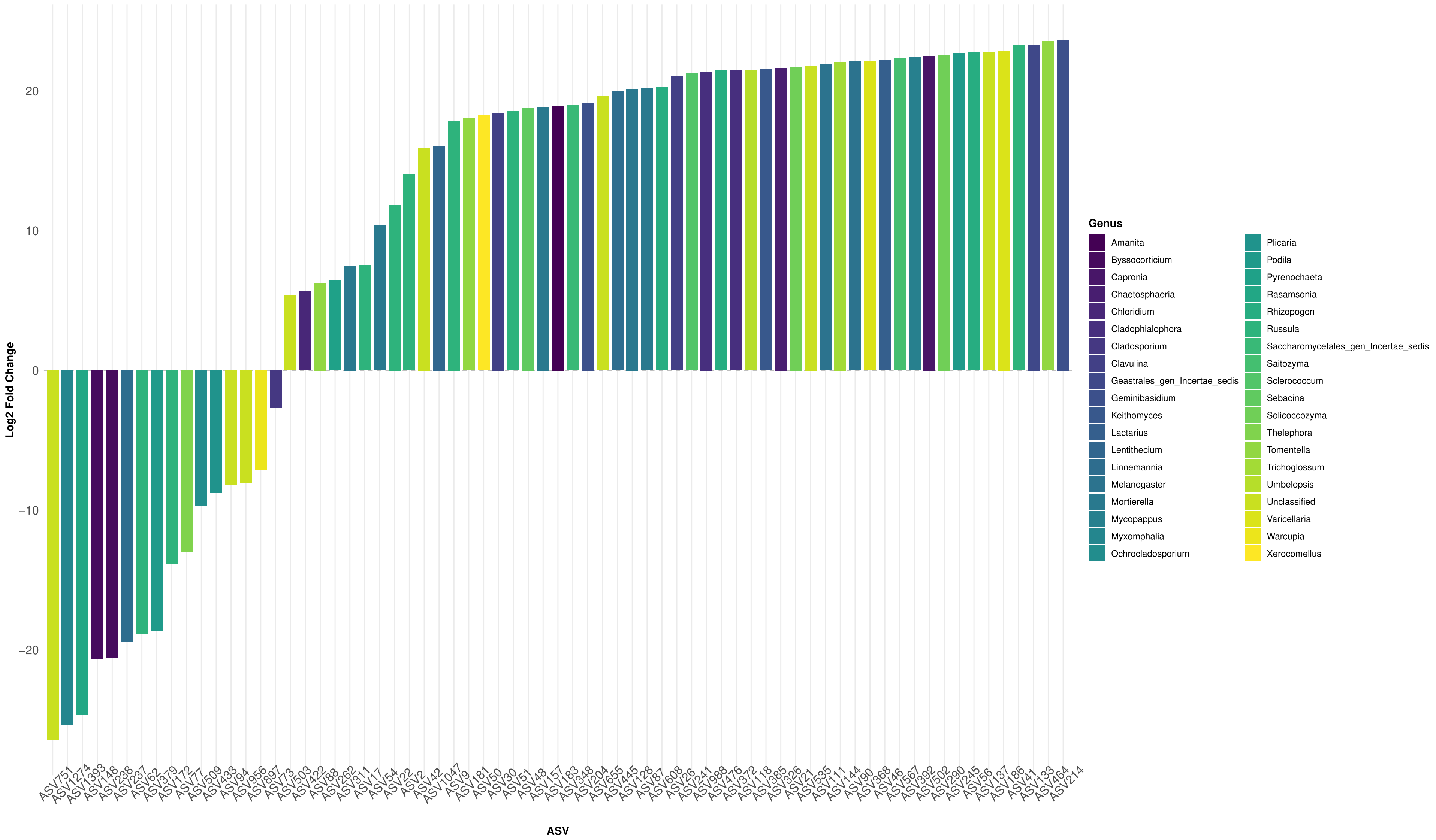
Differential Abundance Analysis: Fire_Mod_SODtrt_vs_wildfire
