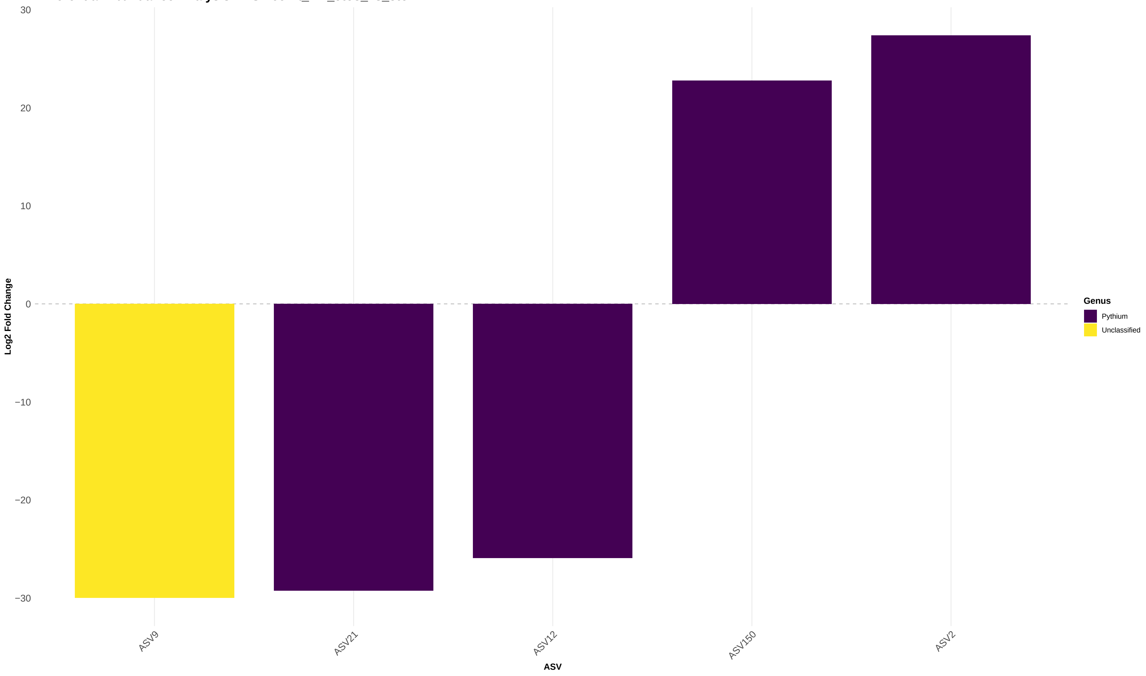
Differential Abundance Analysis: YrSinceTrt_BR_5to8_vs_3to4
