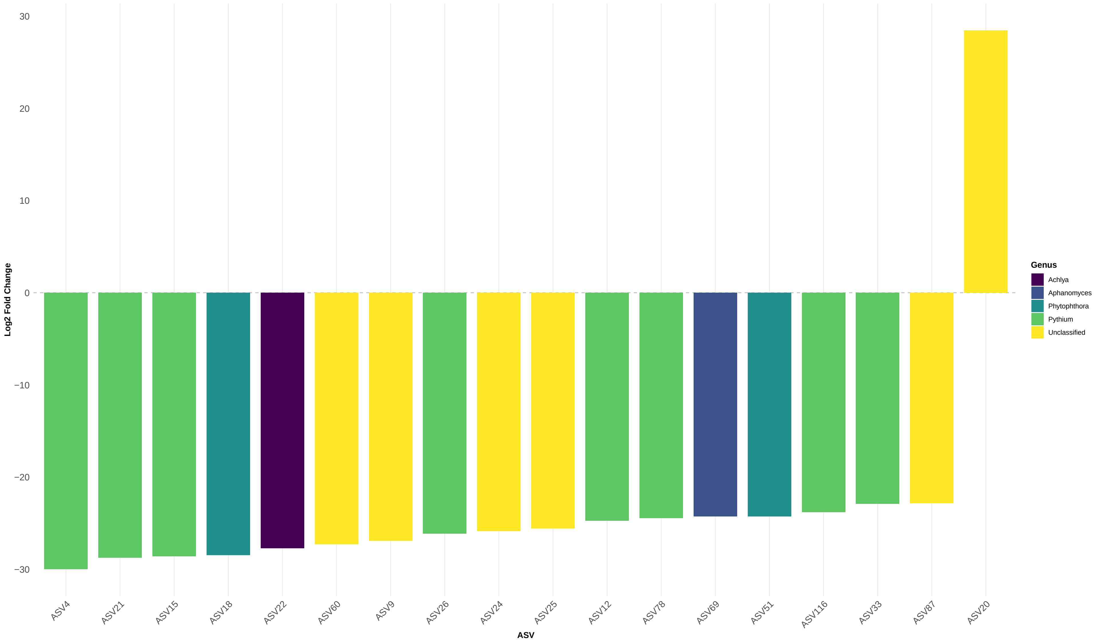
Differential Abundance Analysis: YrSinceTrt_BR_5to8_vs_untreated
