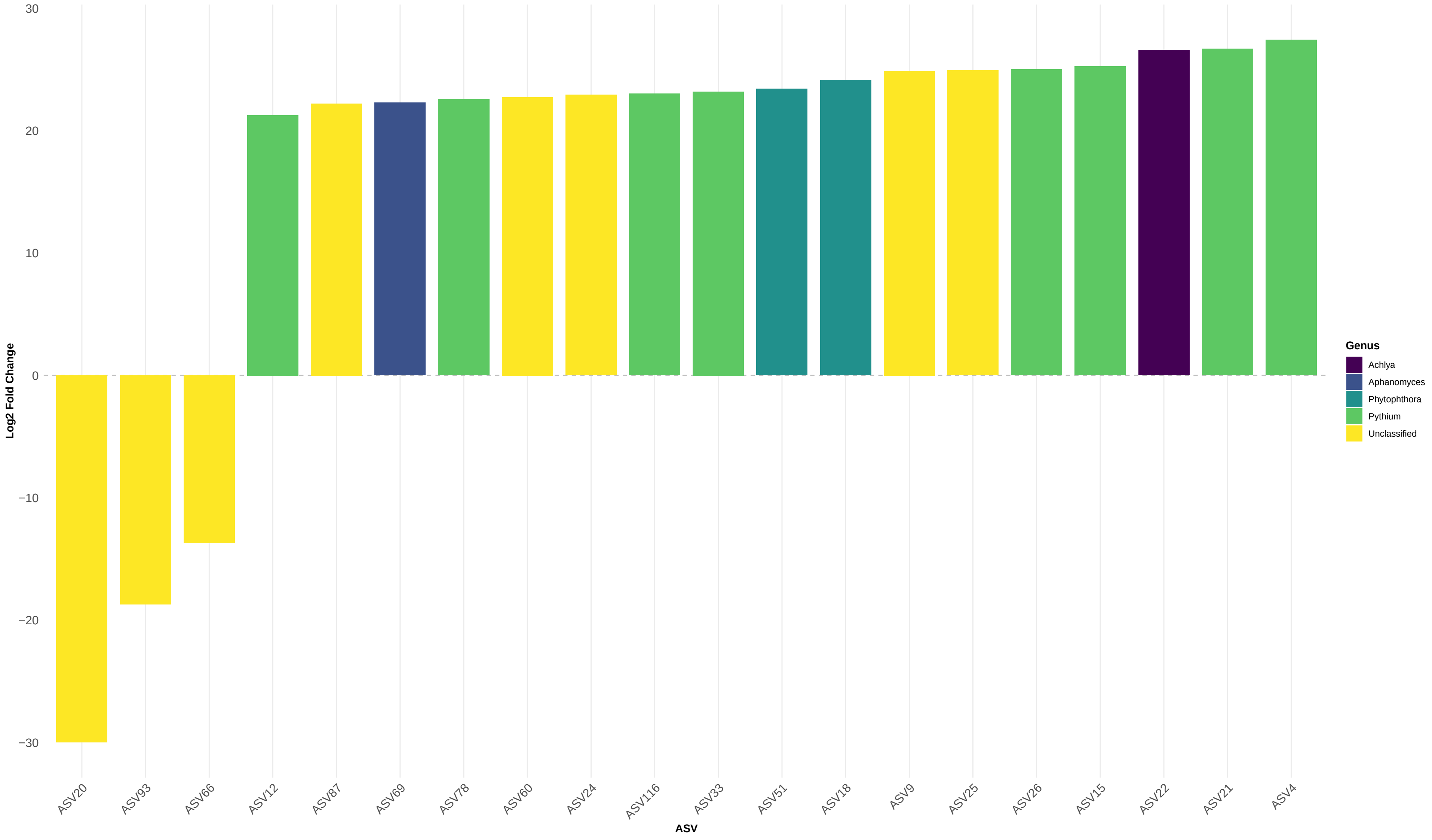
Differential Abundance Analysis: YrSinceTrt_BR_untreated_vs_5to8
