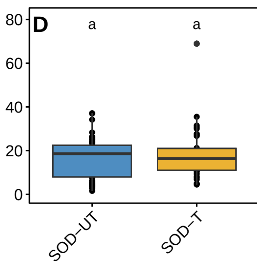
Inverse Simpson Index
