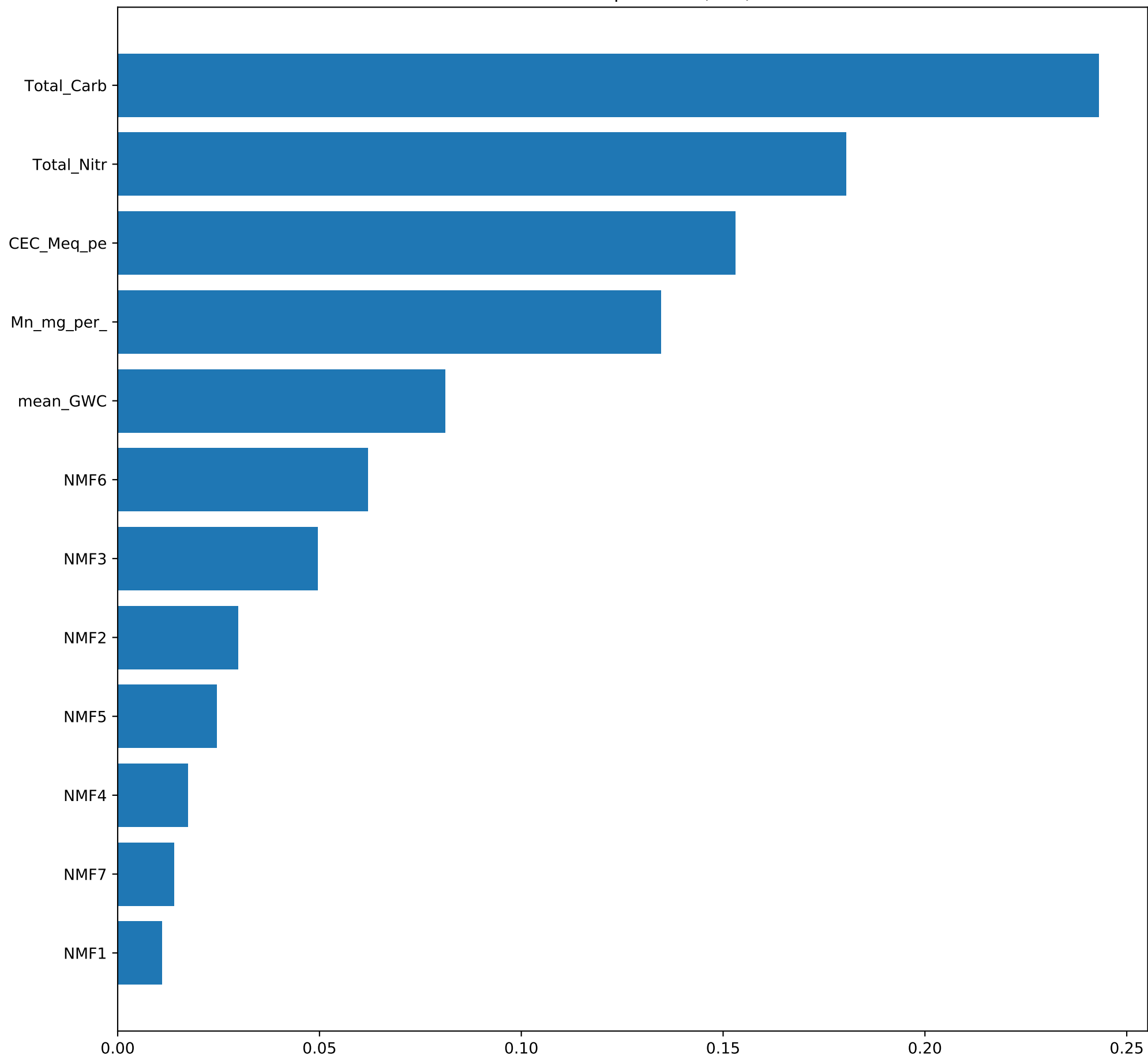
Feature Importance (MDI)
