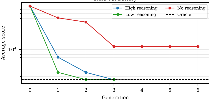
Held-out battery
