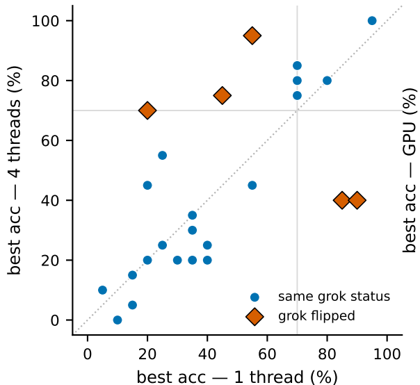
Reduction order (threads): 5/30 flip
