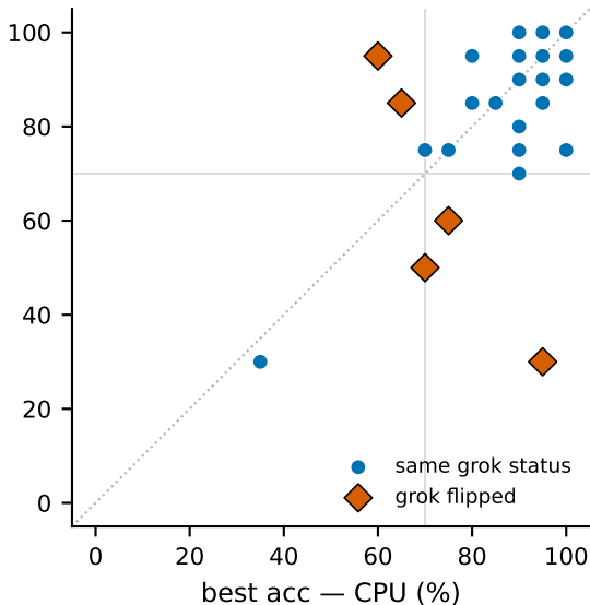
Execution device: 5/30 flip
