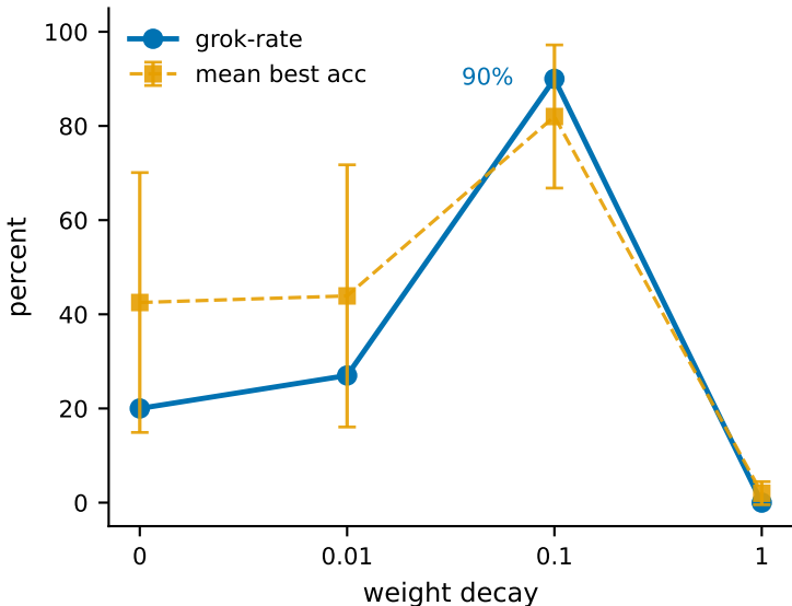
Omnigrok inverted-U at 12K params
