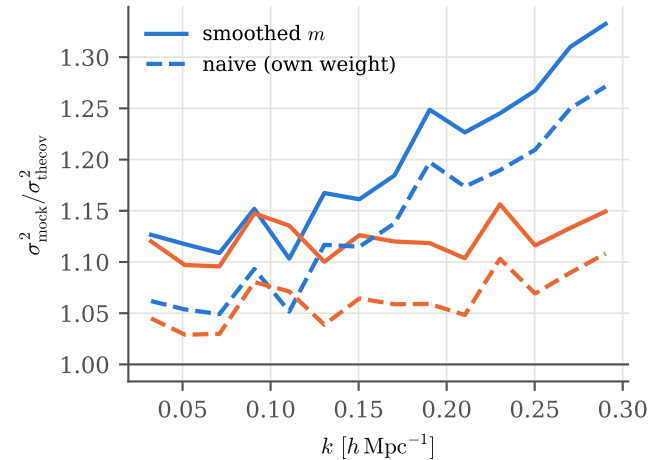
holi LRG1: P_0 (blue), P_2 (orange)
