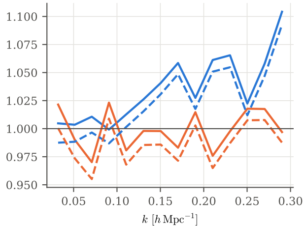
holi QSO: P_0 (blue), P_2 (orange)
