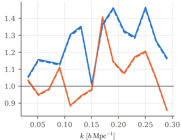
Abacus complete LRG1: P_0 (blue), P_2 (orange)
