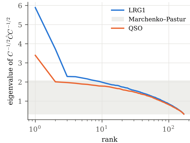
whitened mock covariance (NGC)
