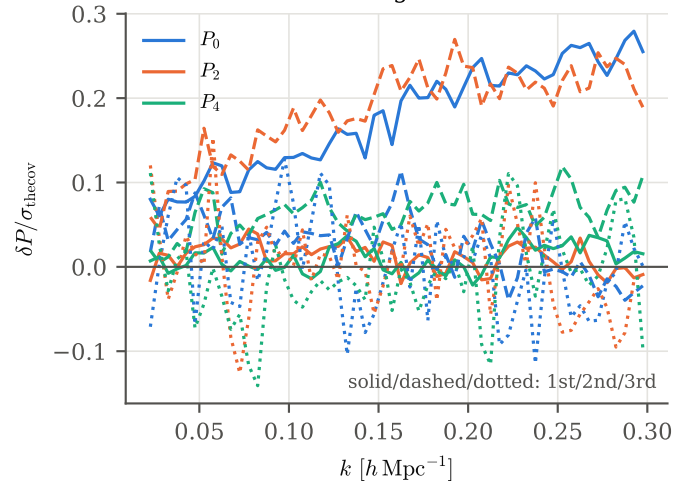
LRG1 NGC: leading excess directions
