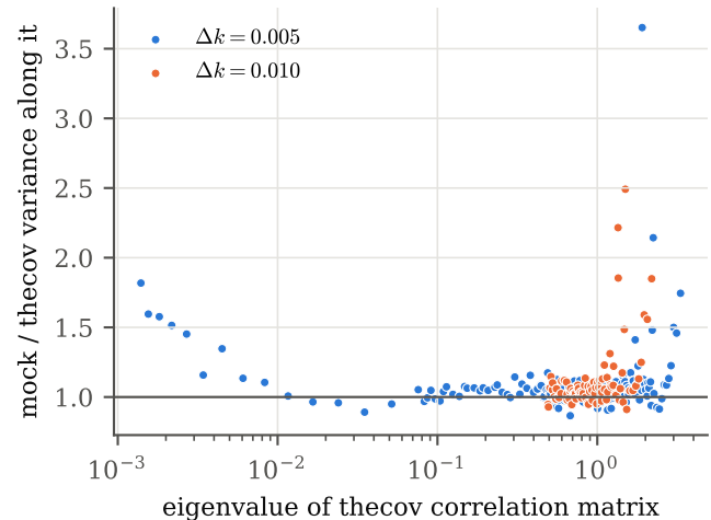
LRG1 NGC: near-null directions
