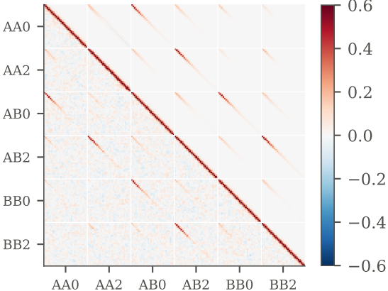
mocks (lower) vs. thecov (upper)
