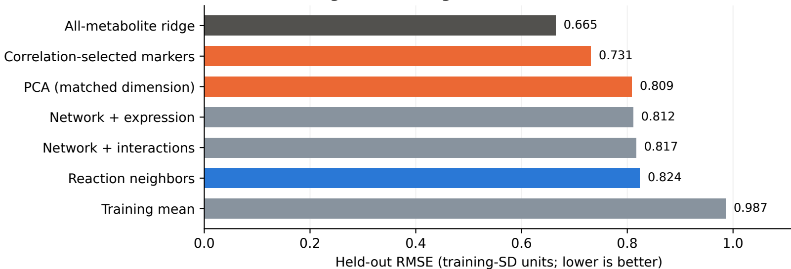
C CCLE · 60 targets, 18 lineages
