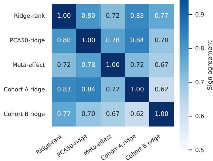
a Method sign agreement (184 contrasts)
