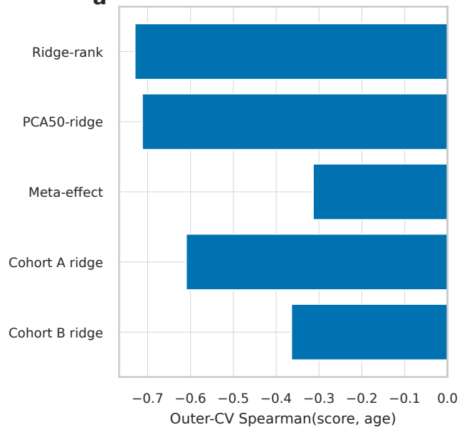
a All evaluable models encode chronological age
