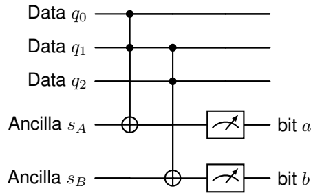
Figure 1.5. Syndrome measurement: The ancilla qubits are activated when the two qubits they monitor are different. Depending on which of the two ancilla qubits are activated, we can determine which of the qubits has flipped.
