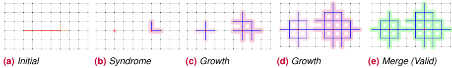
Figure 4.2. Visual representation of the Union-find decoder cluster-growth strategy: edges are data qubits and vertices are the detectors connected to these data qubits. (a) An initial error chain (red) occurs on the lattice, alongside two known erased data qubits (dashed orange), meaning there's prior knowledge of these two data qubits being affected by loss or leakage. (b) The decoder identifies the syndrome defects (red dots) and defines the two odd-parity (invalid) clusters (light and dark magenta). The erased qubits are incorporated to the right cluster. (c) The algorithm grows the clusters uniformly. Because of the initial erasures, the right cluster expands faster. (d) In the second growth step, the boundaries of both clusters collide at a shared node. (e) This collision immediately triggers a union operation. The newly merged cluster now contains an even number of defects, changing its overall status to valid (green) and halting the growth phase.
