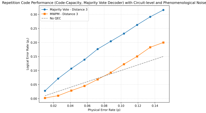
Figure 5.2. Simulation 4: Impact of circuit-level and phenomenological noise on the repetition code performance. Introducing more complex noise significantly degrades the logical error suppression compared to the idealized code-capacity baseline. With this additional noise, MWPM shows its advantage over the Majority Vote because of its capacity to consider the probabilities of each error to select the most probable set of errors that could have caused the observed syndrome.
