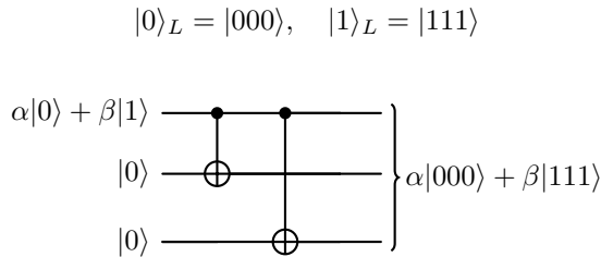
Figure 1.4. Encoding circuit for the bit-flip code. Entanglement distributes the logical information without violating the no-cloning theorem.
