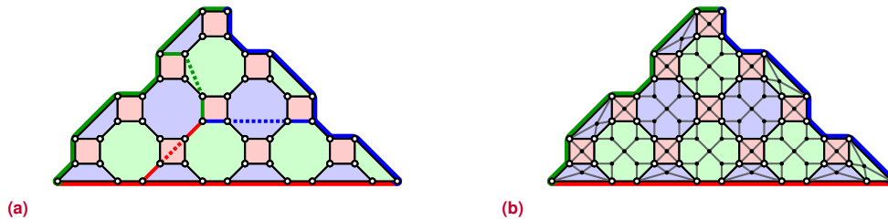
Figure 2.4. Planar topology of a 4.8.8 lattice color code. (a) Definition of the triangular patch for a planar topology, in which we must use string-nets to define the logical observables. Each string-net can encode the logical X and Z operators in the color code, but the individual strings must terminate at a boundary of their own color, which inherently requires branching. (b) Mapping of the color code patch to a quantum processor with a square grid of qubits. For the octagonal faces, we must use 5 ancillas to perform the stabilizer measurements. Ancilla qubits in the tetrahedrons that appear in the boundaries do not map the square grid and are intentionally simplified in this diagram.
