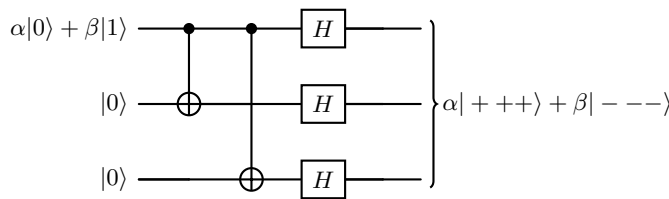
Figure 1.6. Encoding circuit for the 3-qubit phase-flip code. The information is first distributed via entanglement, and then Hadamard gates transform the final state into the \{|+\rangle, |-\rangle\} basis.
