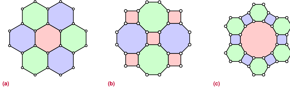
Figure 2.2. The three valid 2D configurations for topological color codes: the 6.6.6 hexagonal lattice, the 4.8.8 square-octagonal lattice, and the 4.6.12 lattice. The faces are 3-colored (e.g., red, green, blue) such that no two adjacent faces share the same color. Data qubits are represented with white circles. There are two ancilla qubits in each colored face, which are not represented in the image.
