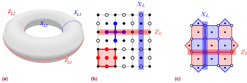
Figure 2.1. Evolution and representations of the surface code. (a) The toric code representation, illustrating how logical observables correspond to non-contractible continuous strings wrapping around the two fundamental cycles of the torus. (b) The original planar formulation by Kitaev ( d = 4 ), with data qubits on the edges and checks on vertices and faces. The red square represents a Z -stabilizer and the blue cross represents a X -stabilizer. A total of 49 physical qubits are needed. (c) The equivalent rotated surface code, placing data on vertices and alternating checks on colored faces to significantly reduce physical overhead. Red faces represent Z -stabilizers and blue faces represent X -stabilizers. The blue and red lines represent the minimum string for the respective operators. In this case, only 31 physical qubits are required. In figures (b) and (c) for a d = 4 code, white circles represent data qubits and black circles represent ancilla qubits. The blue and red lines represent the minimum strings for the respective logical operators.
