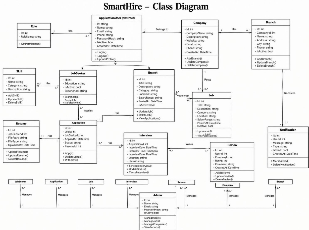
Figure 6.16: Class Diagram for
