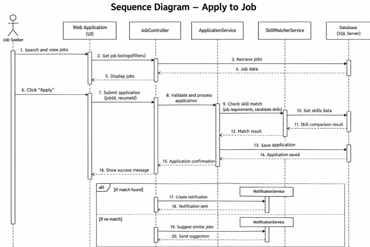
Figure 6.15: Sequence Diagram for Applying Job
