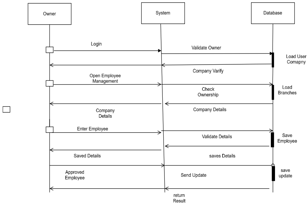
Figure 6.7: Swim Lane Diagram for Company owner add employee
