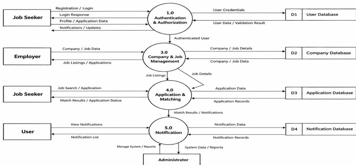
Figure 6.12: Level-1 Data Flow Diagram
