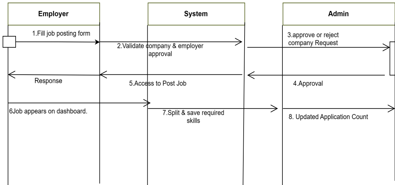
Figure 6.9: Swim Lane Diagram for Job Posting
