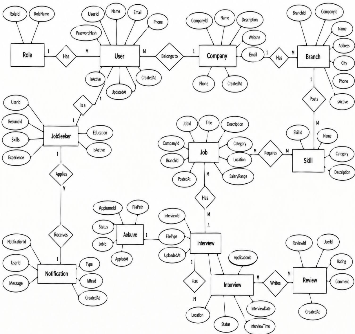
Figure 6.17: SmartHire Entity Relationship Diagram (ERD)
