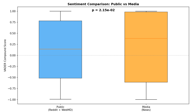
Figure 1: Sentiment comparison between public and media corpora (hybrid mode).
