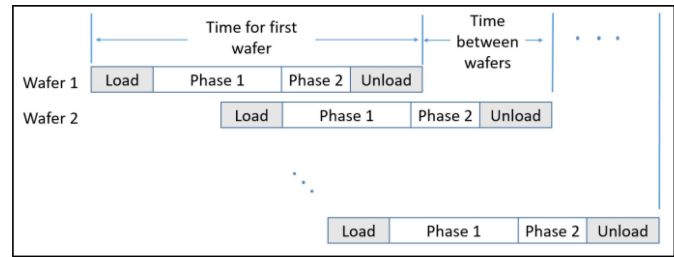
Fig. 1. Wafer cascading.
