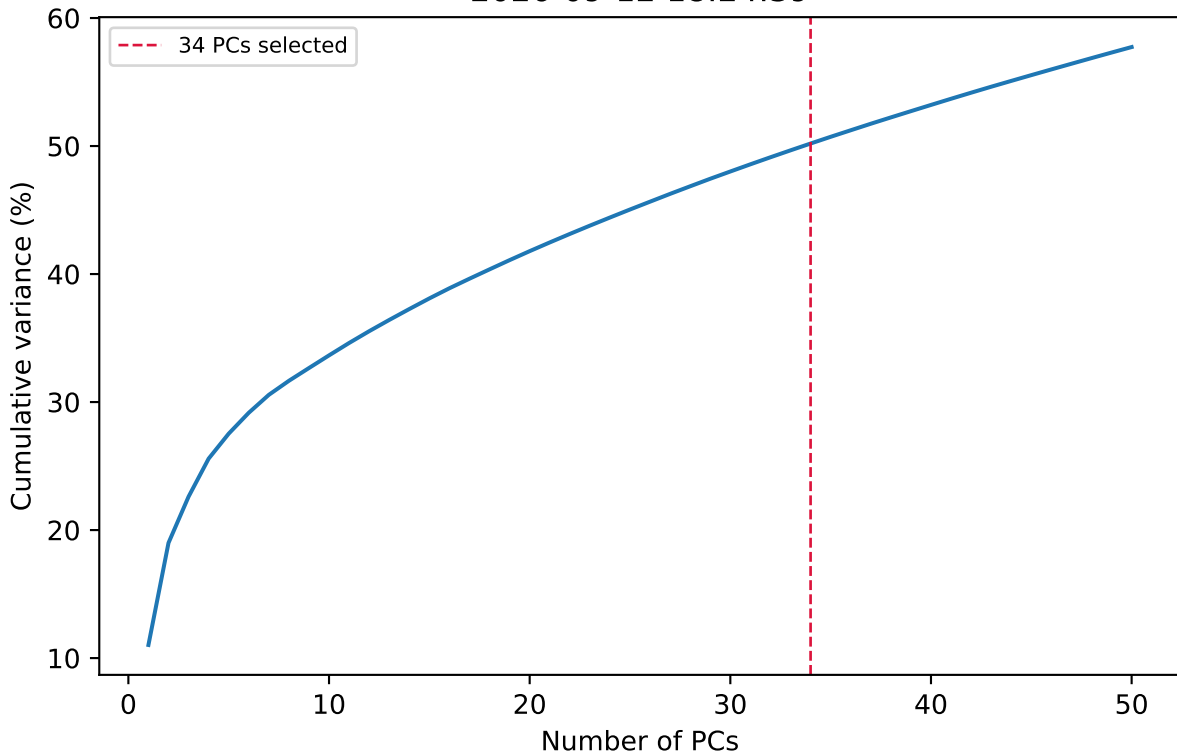
Cumulative Variance by PCs Dataset: SRX23395189 (cell_type) 2026-09-12 18:24:39
