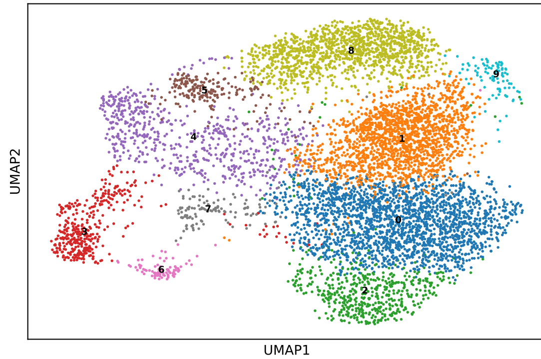
Leiden 0.8 (10 clusters)
