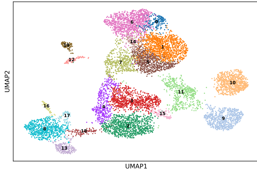
Leiden 1.0 (20 clusters)
