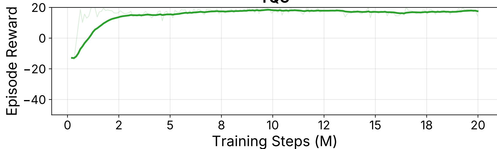
TQC
